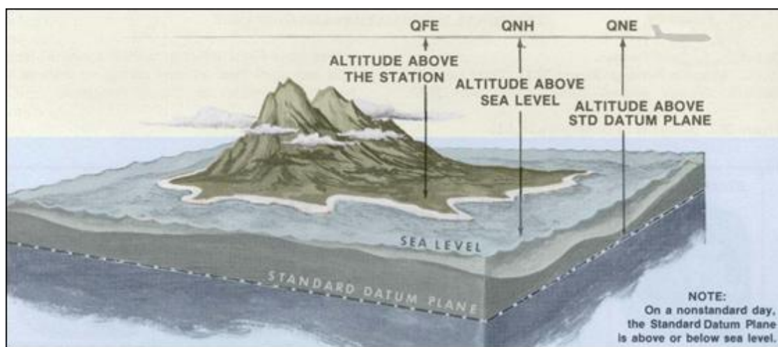
Figure 4.8. Types of Altimeter Settings.
