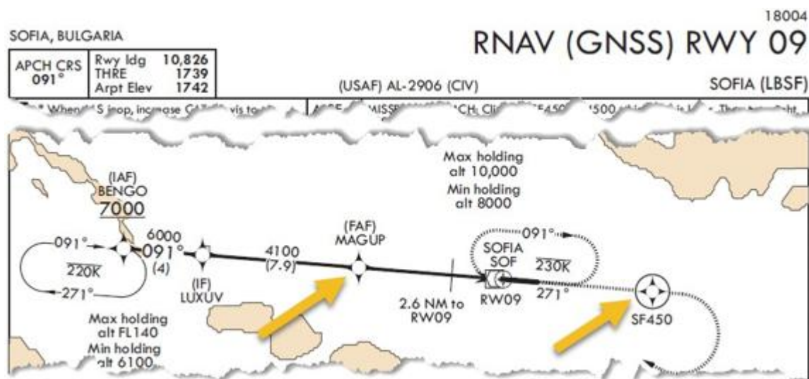
Figure 10.3. Fly-by versus Fly-over Waypoint.
