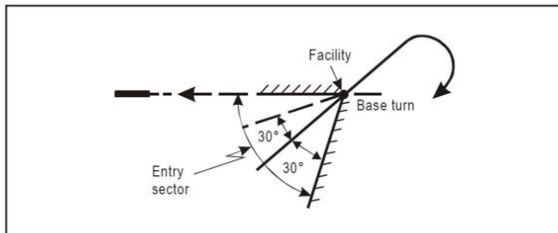
Figure 15.15. Base Turn Entry Expanded Entry Sector.
