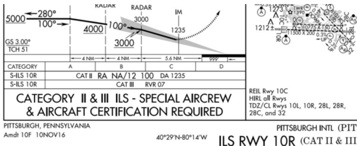
Figure 17.2. CAT II ILS Approach.
