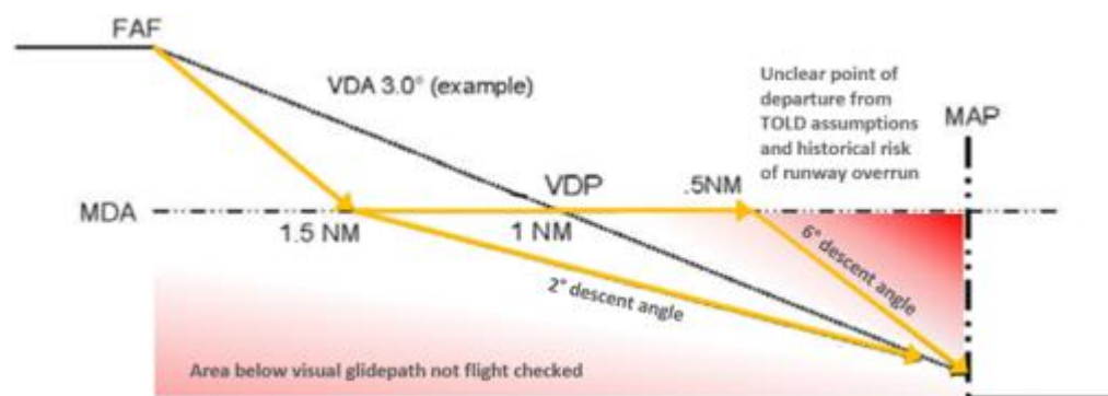
Figure 16.4. Dive and Drive.
