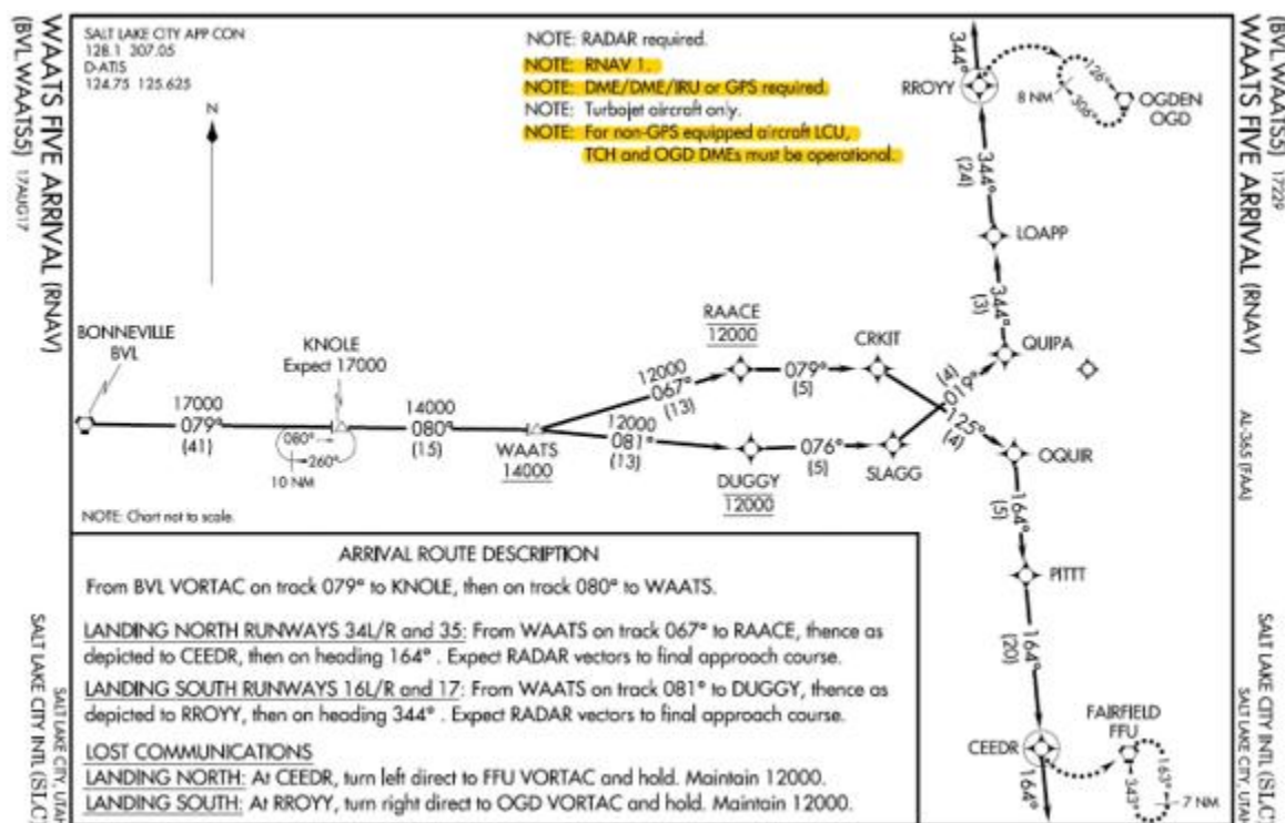
Figure 14.1. RNAV Arrival.
