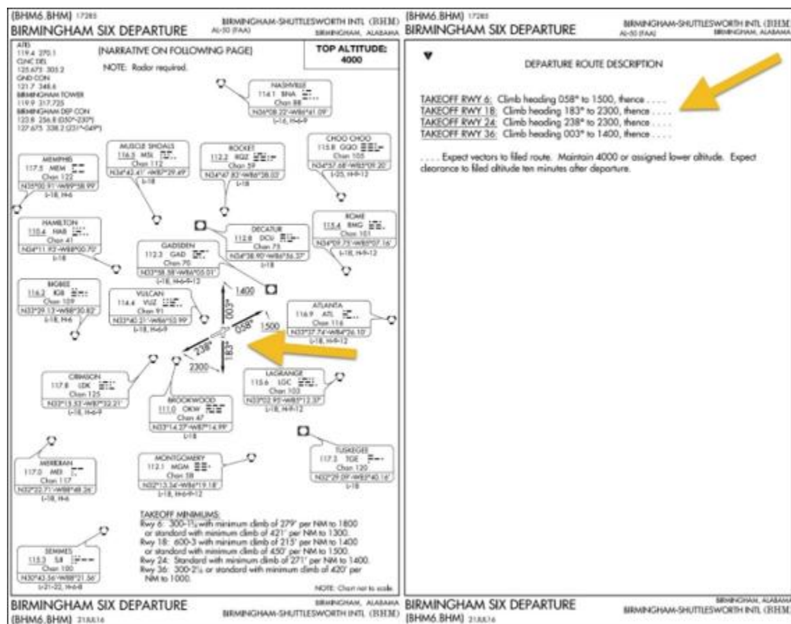
Figure 5.28. Radar Vector SID.
