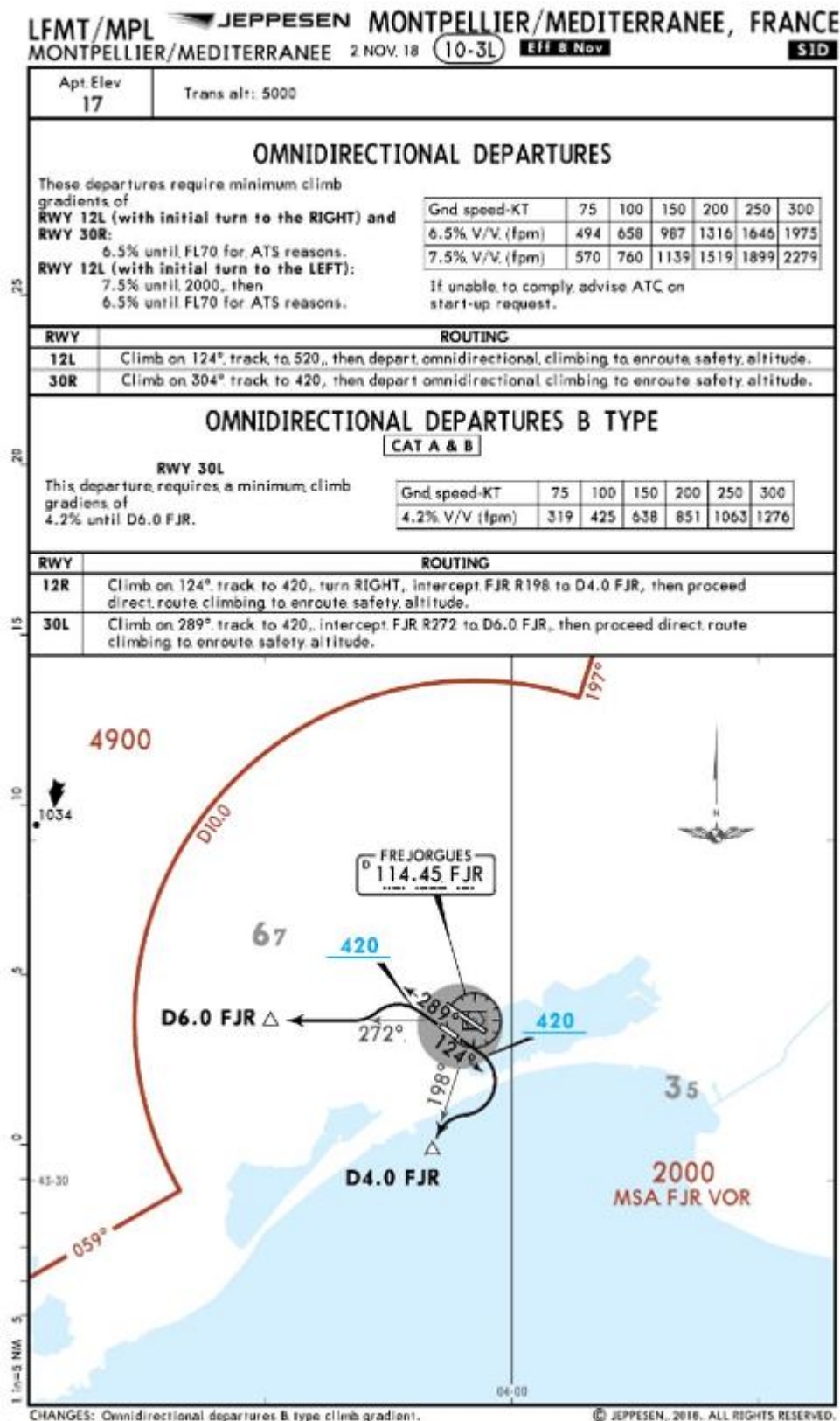
Figure 5.6. Example Omnidirectional Departure.
