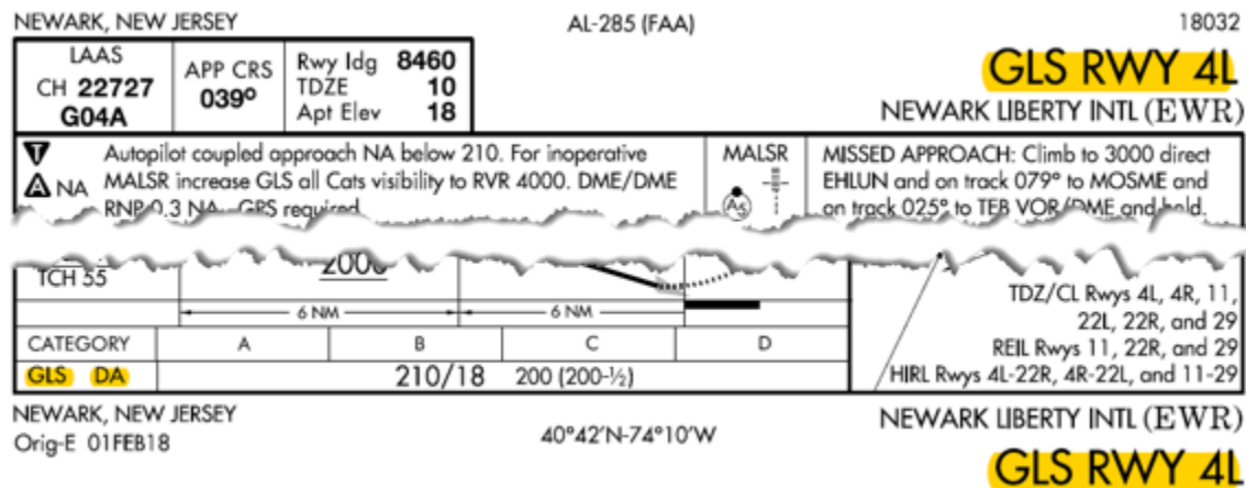
Figure 9.1. GBAS Landing System (GLS) Approach.
