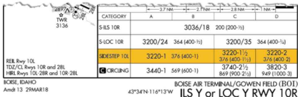
Figure 18.5. Published Side-Step Minima.
