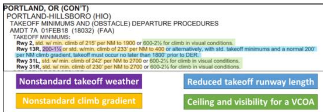
Figure 5.8. Example Nonstandard IFR Takeoff Minimums on SID in the NAS.
