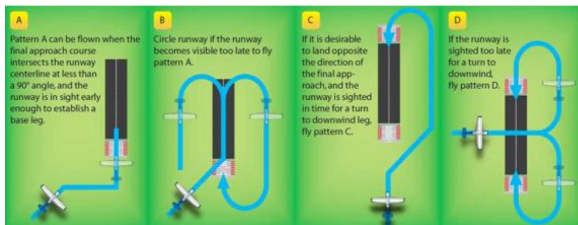
Figure 18.3. Circling Maneuver Examples.
