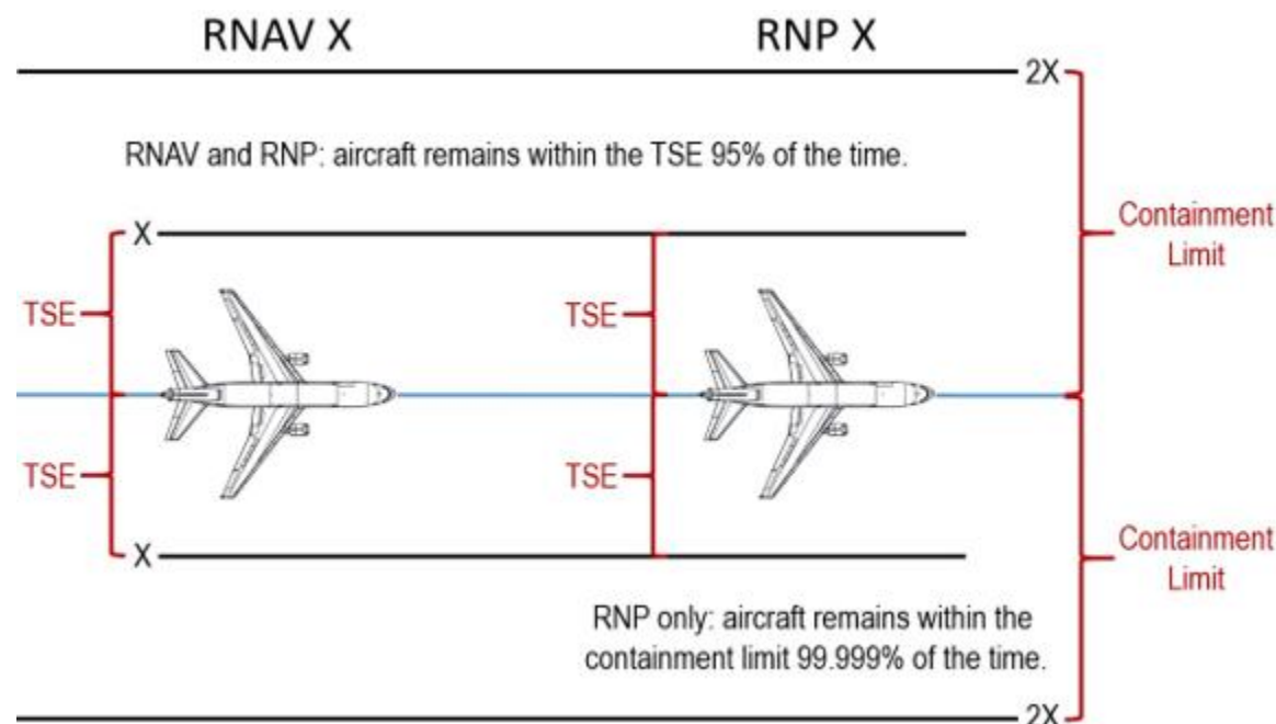
Figure 6.4. RNAV Designations vs RNP Designations.
