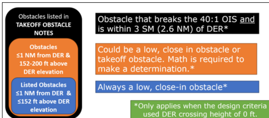
Figure 5.2. TAKEOFF OBSTACLE NOTES Generalization.
