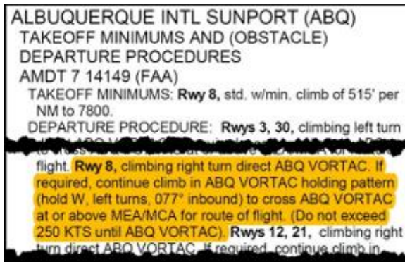
Figure 5.31. Albuquerque SDP (Runway 8).
