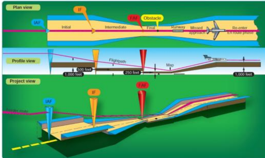
Figure 15.10. Approach Segments.
