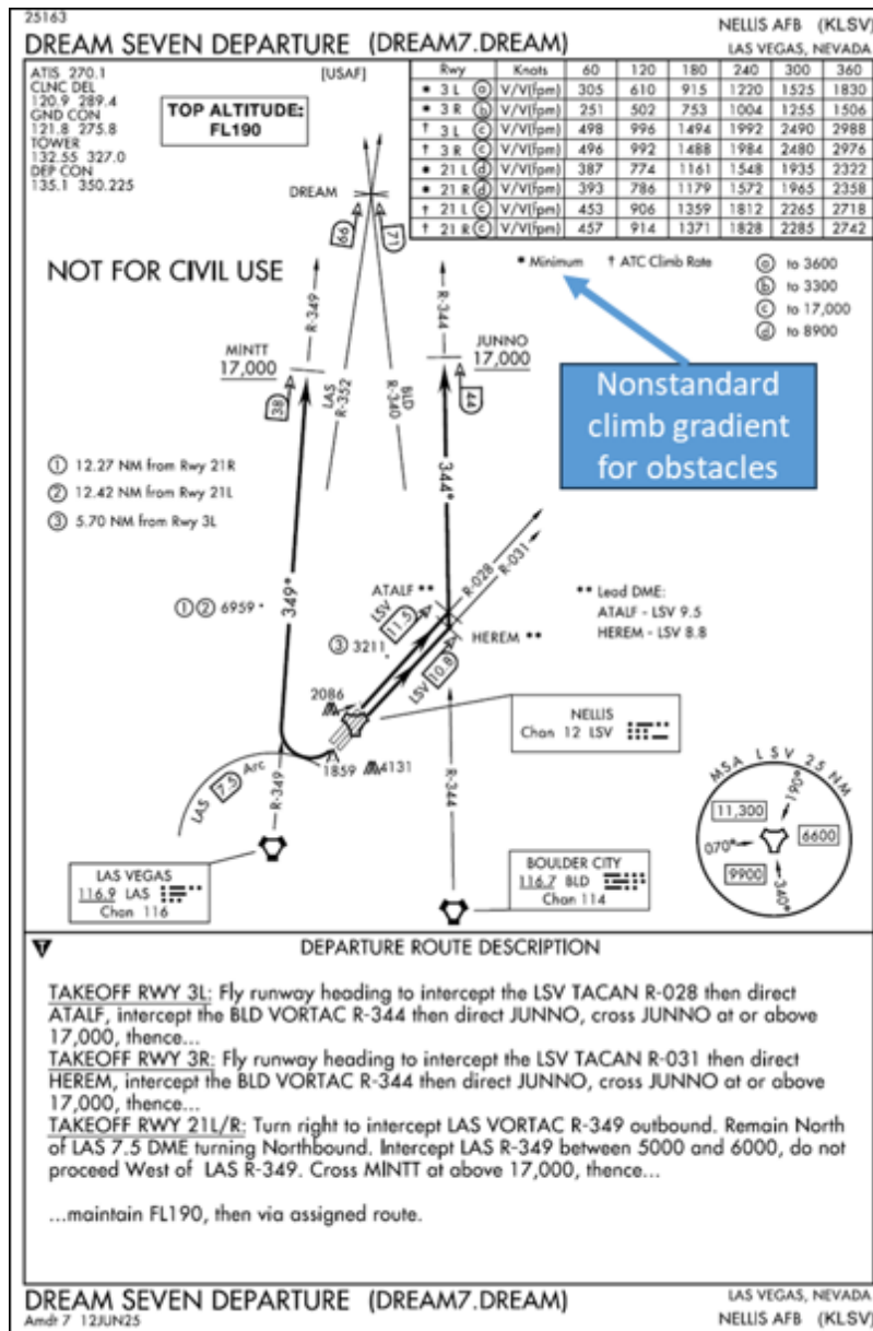
Figure 5.26. Military SID.
