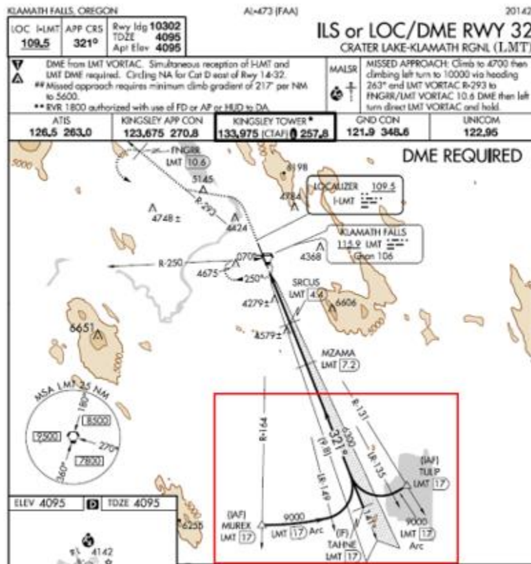
Figure 15.18. Procedure Turn Not Authorized.
