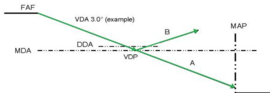
Figure 16.5. CDFA.
