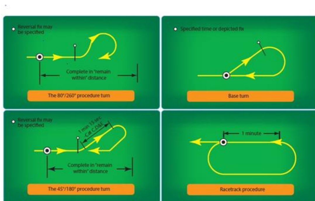
Figure 15.13. Types of Course Reversals.
