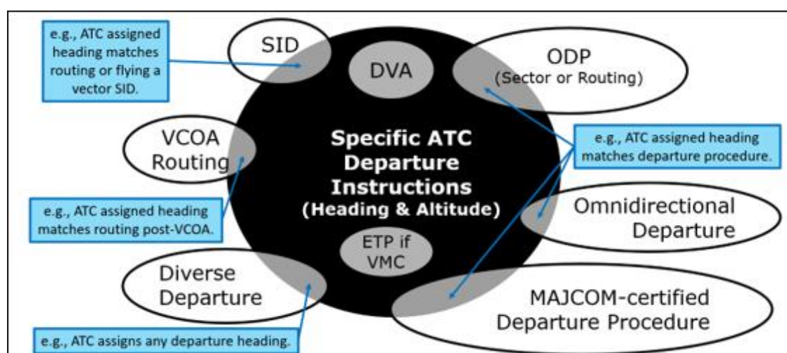
Figure 5.23. Combination of Departure Procedures.
