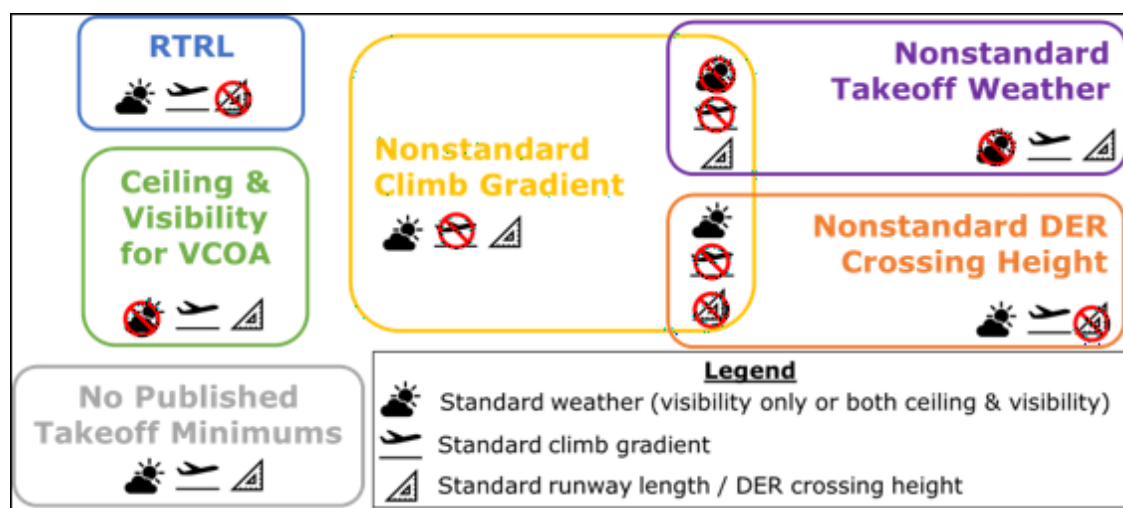
Figure 5.22. Combination of Standard and Nonstandard Takeoff Minimums.
