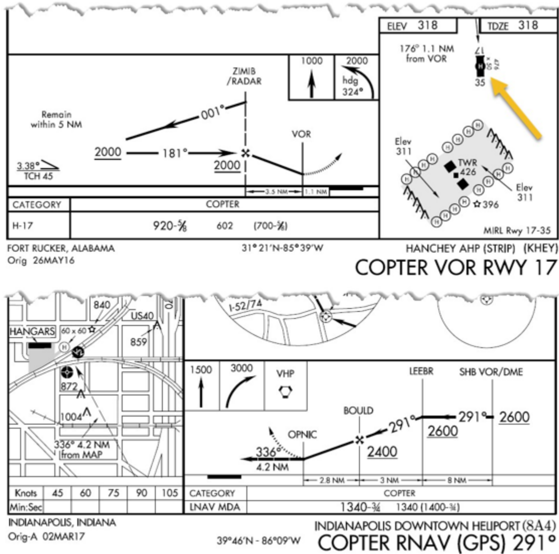
Figure 15.30. Helicopter-Only Approach.
