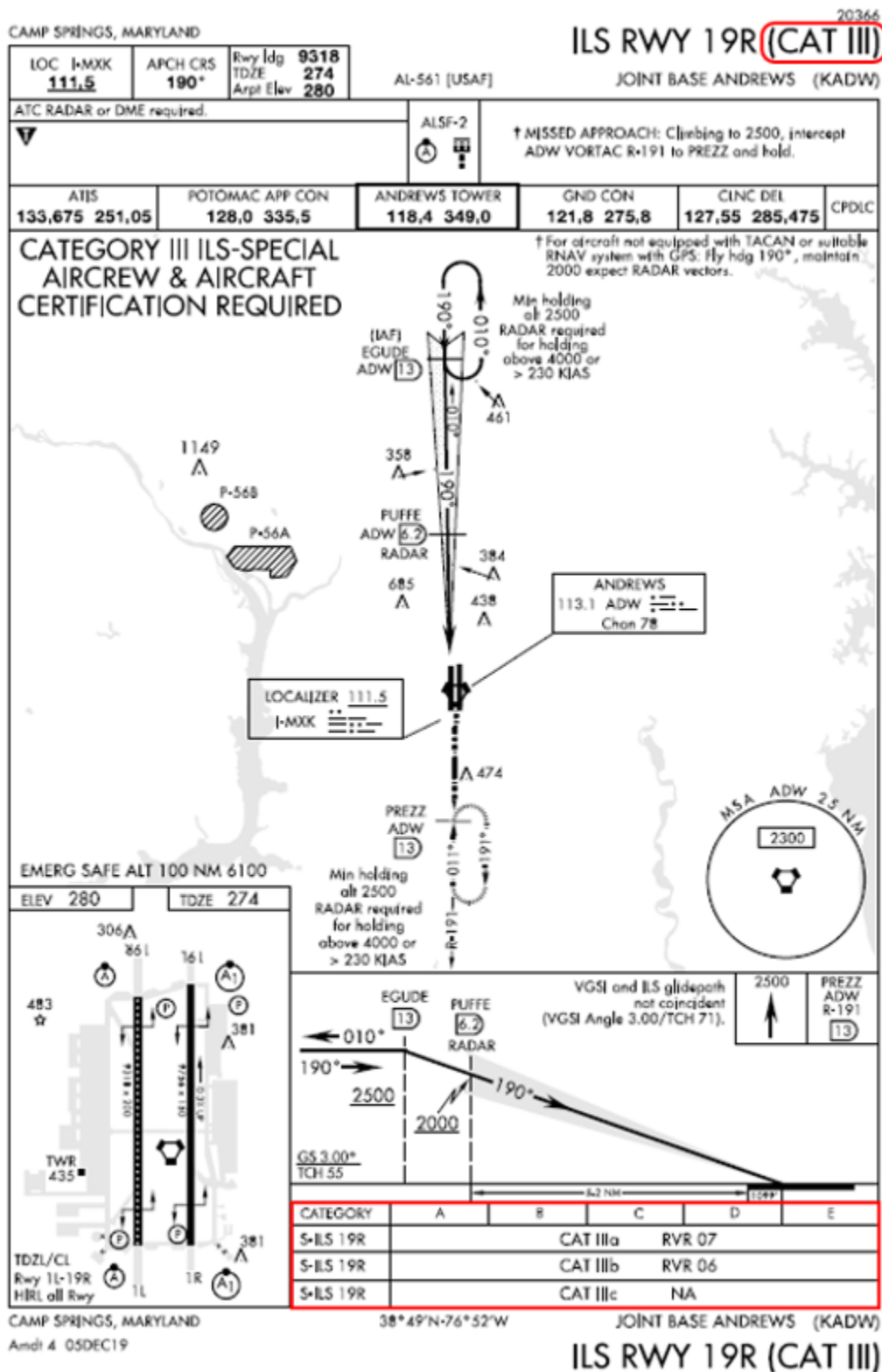
Figure 17.5. CAT III ILS Approach.
