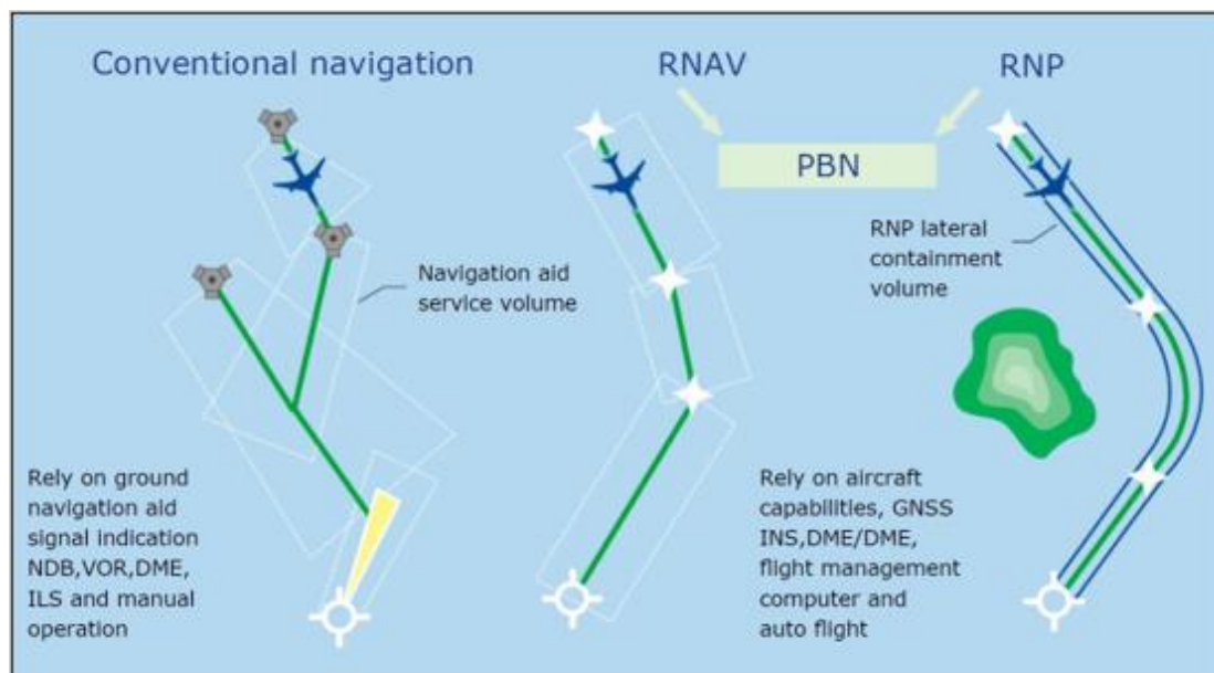
Figure 6.1. Progression from Sensor-based to Performance-based Navigation.
