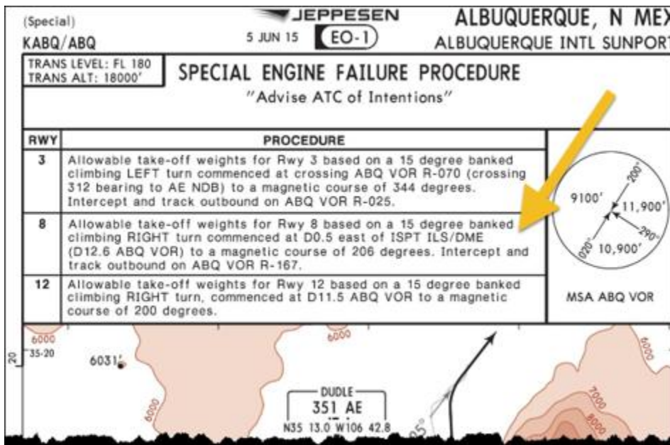
Figure 5.31. Albuquerque SDP (Runway 8).
