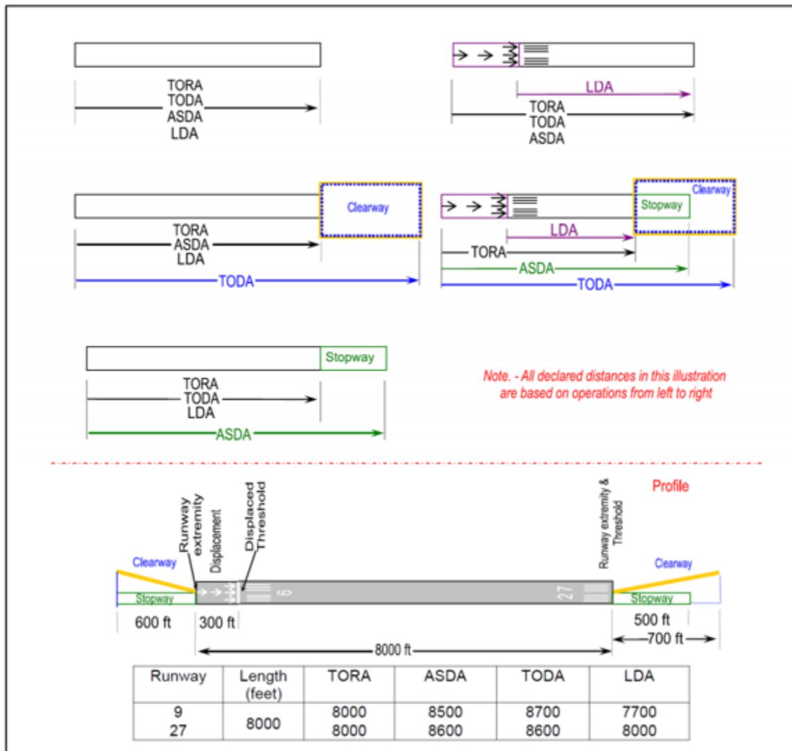
Figure 4.6. {NAS Only} Declared Distances.
