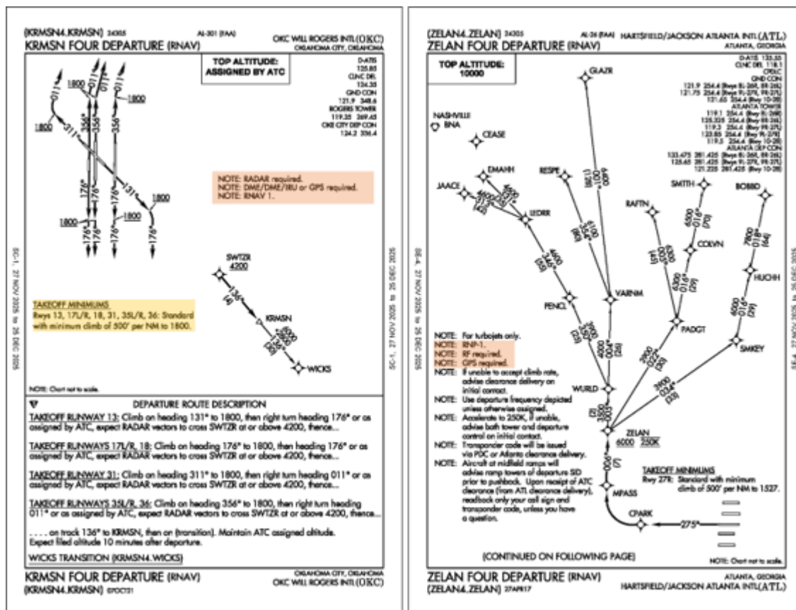
Figure 5.29. Example PBN SIDs.
