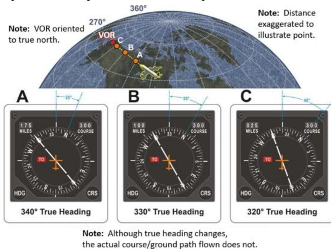
Figure 20.1. Heading Indications While Crossing Meridians.
