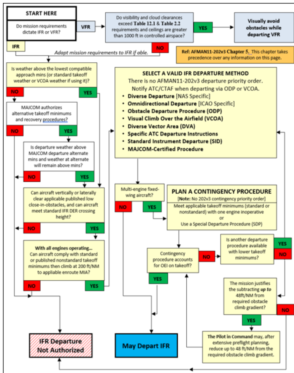
Figure A8.1. Departure Decision Tree.
