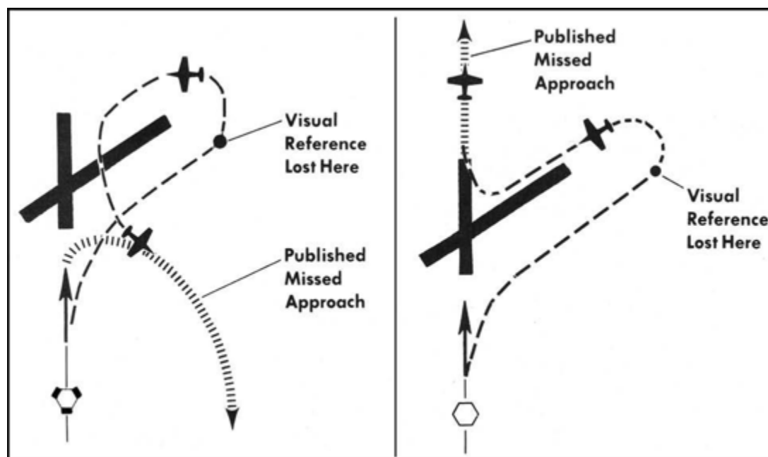
Figure 19.2. Missed Approach from the Circling Approach.
