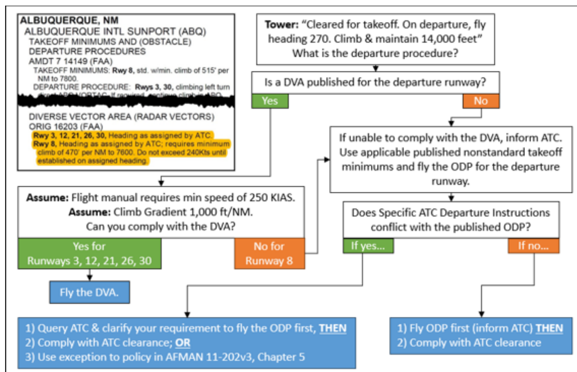
Figure 5.24. Example DVA and Flow Chart.
