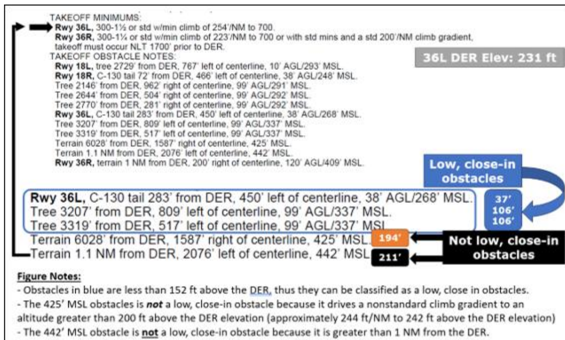
Figure 5.3. TAKEOFF OBSTACLE NOTES Classification Example.
