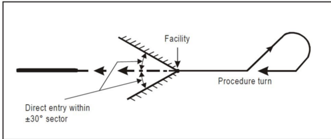
Figure 15.14. Direct Entry Sector.
