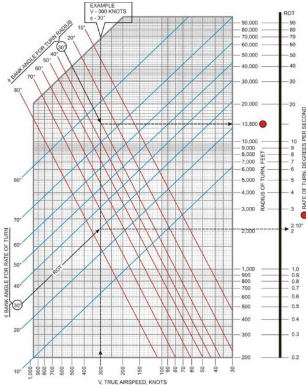
Figure A3.1. General turning performance (constant altitude, steady turn).
