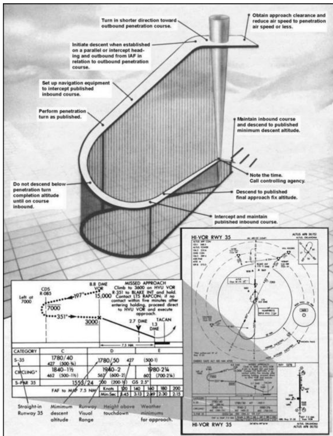
Figure 15.29. Non-DME Teardrop High Altitude Approach.
