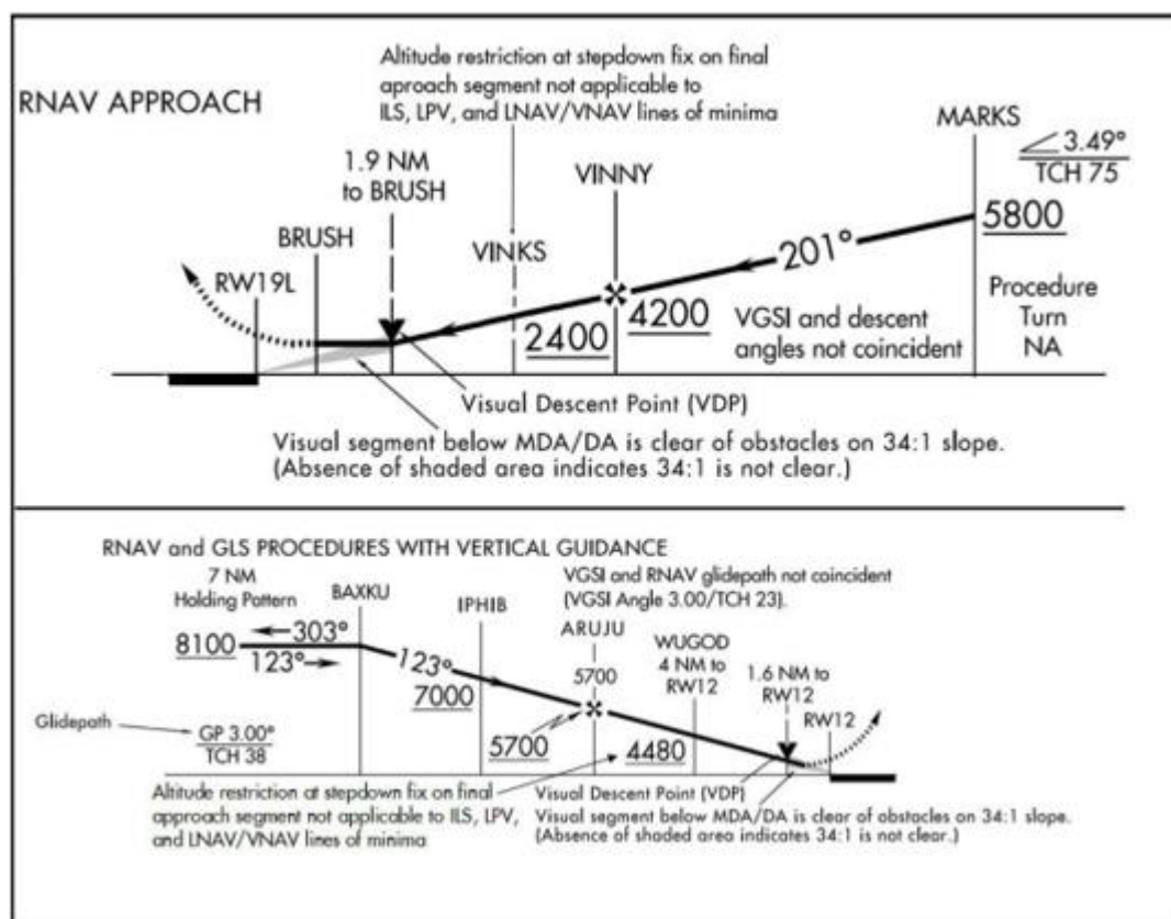
Figure 15.28. Instrument Procedure Stepdown Fixes.
