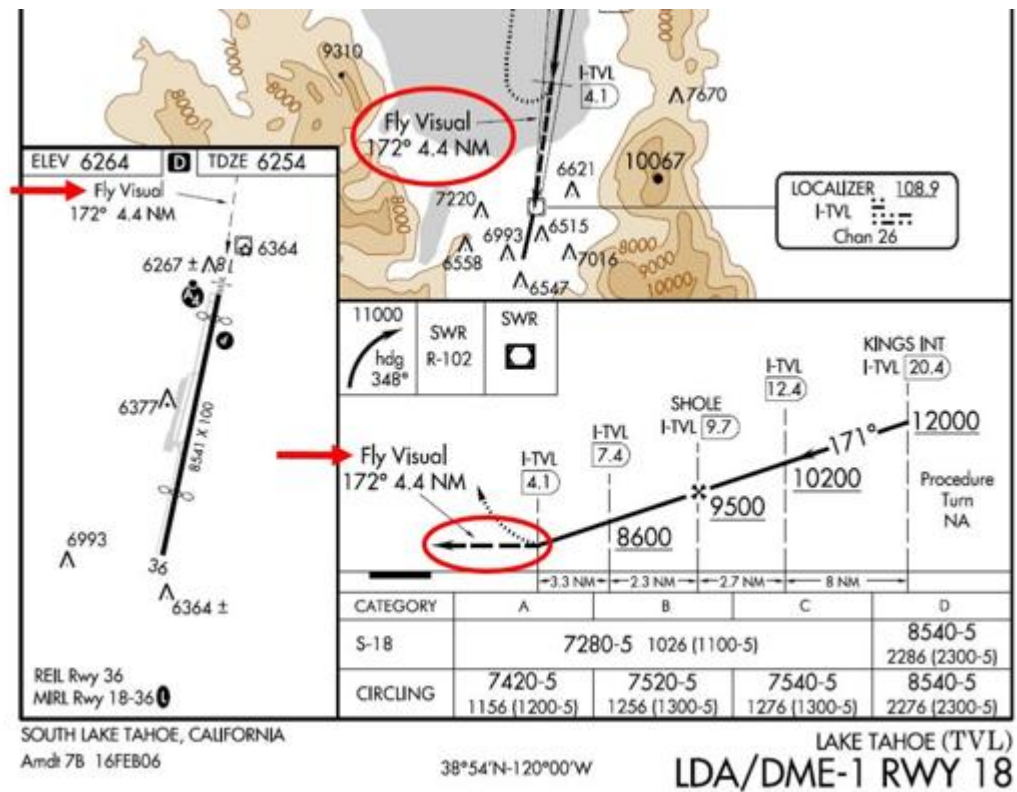
Figure 16.10. Visual Segment.
