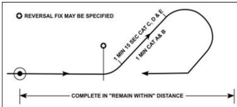
Figure 15.21. 45°/180° Procedure Turn.
