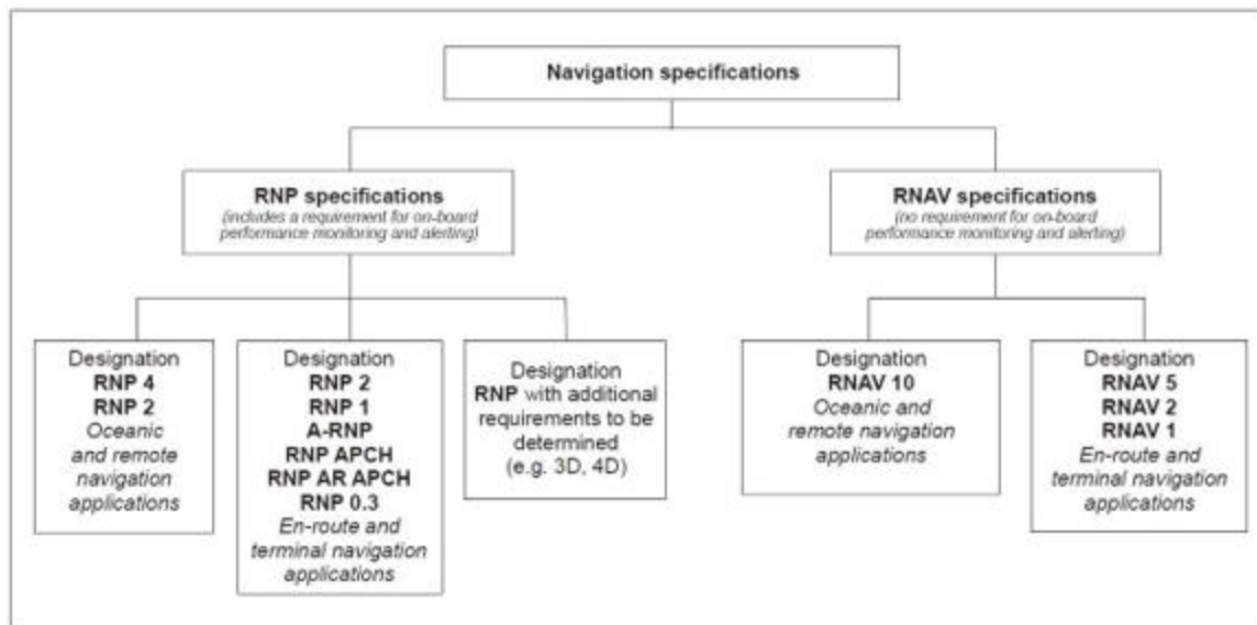
Figure 6.2. Navigation Specification Designations.
