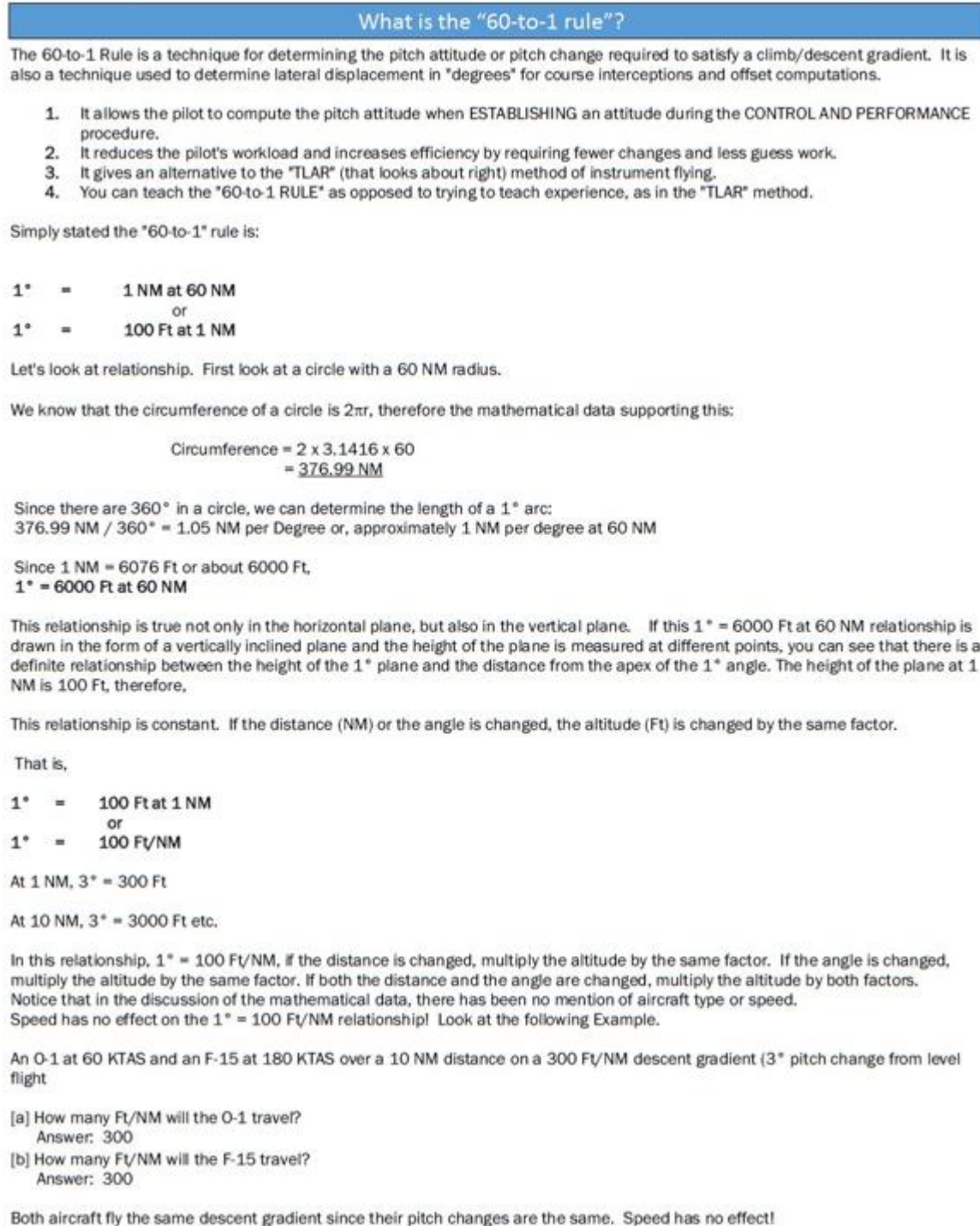
Figure A2.1. The "60-to-1 Rule." (Page 1 of 2)
