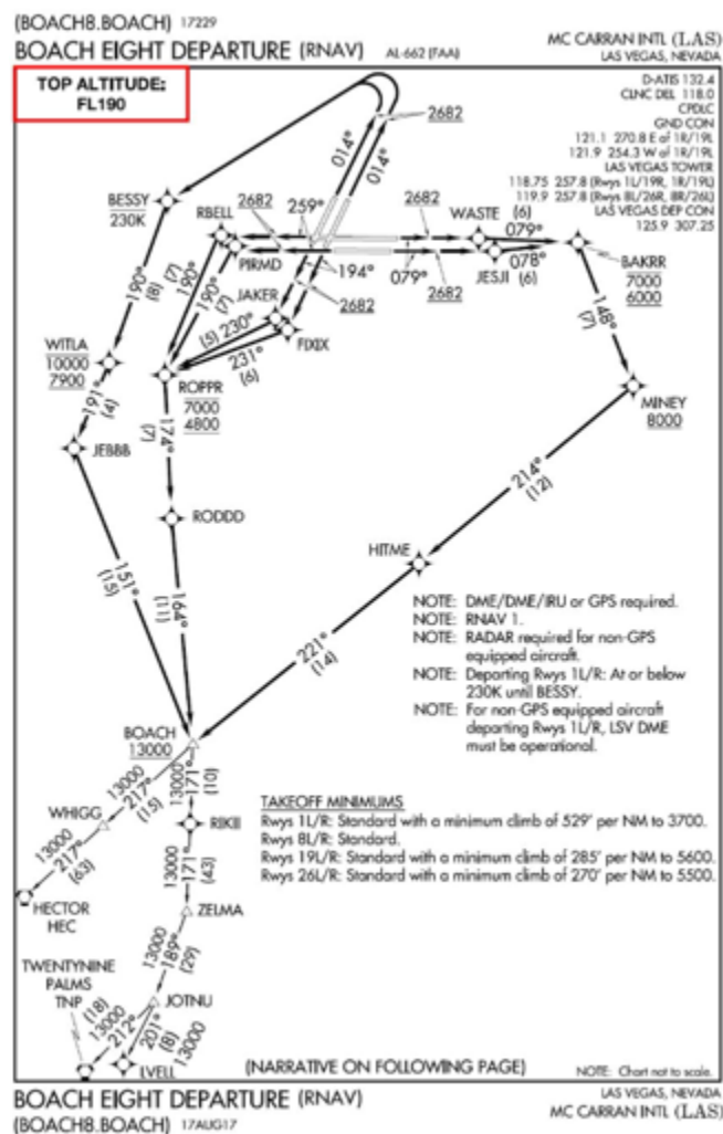
Figure 5.25. Civil SID with Top Altitude.
