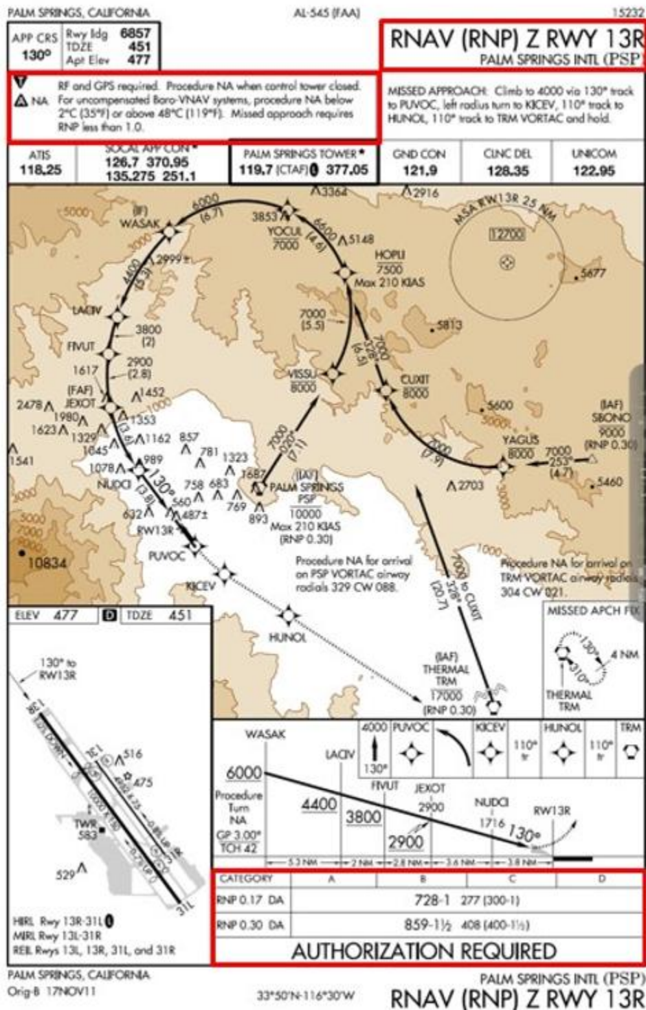
Figure 17.6. RNP Values.
