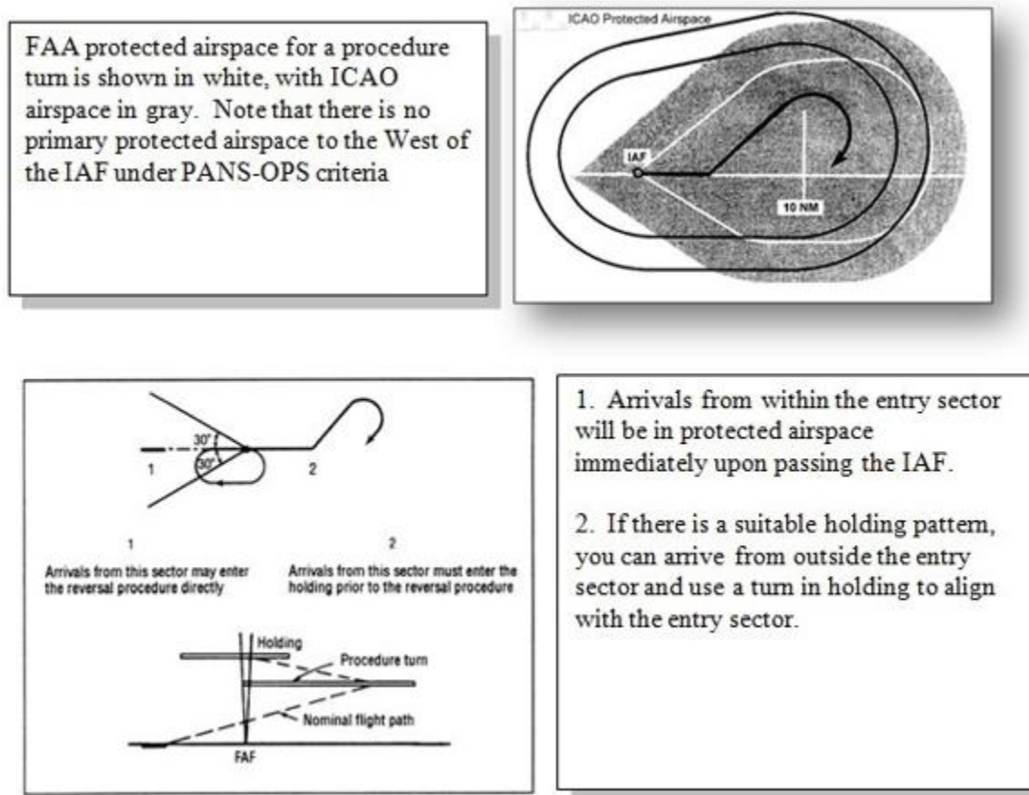
Figure 15.16. ICAO PANS-OPS versus U.S. TERPS Protected Airspace.
