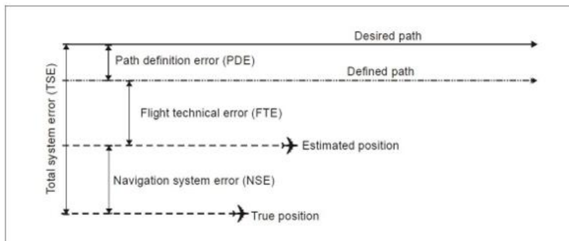
Figure 6.3. Lateral Navigation Errors.
