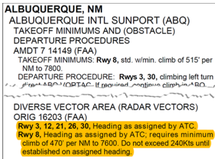
Figure 5.18. Diverse Vector Area.
