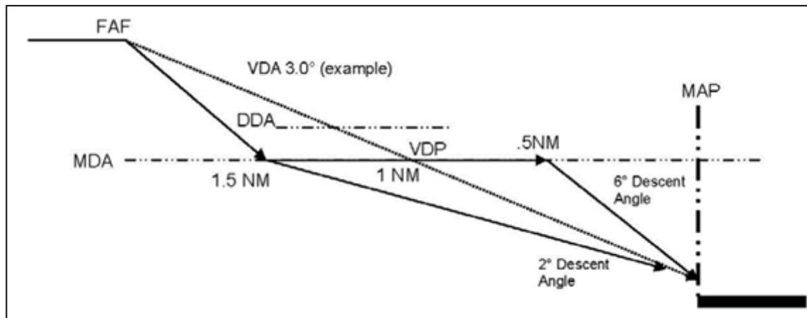
Figure 16.4. Dive and Drive.
