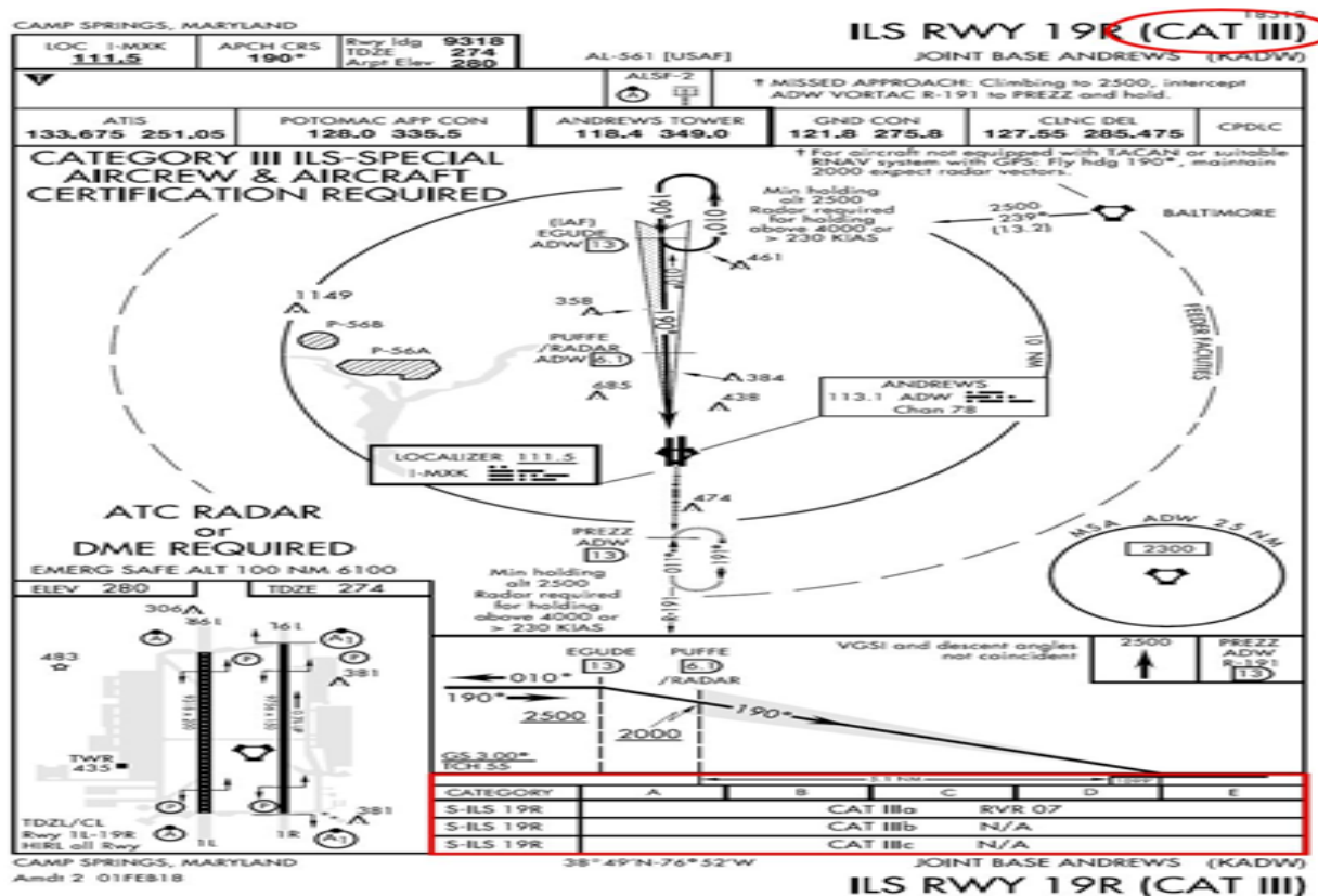
Figure 17.5. CAT III ILS Approach.
