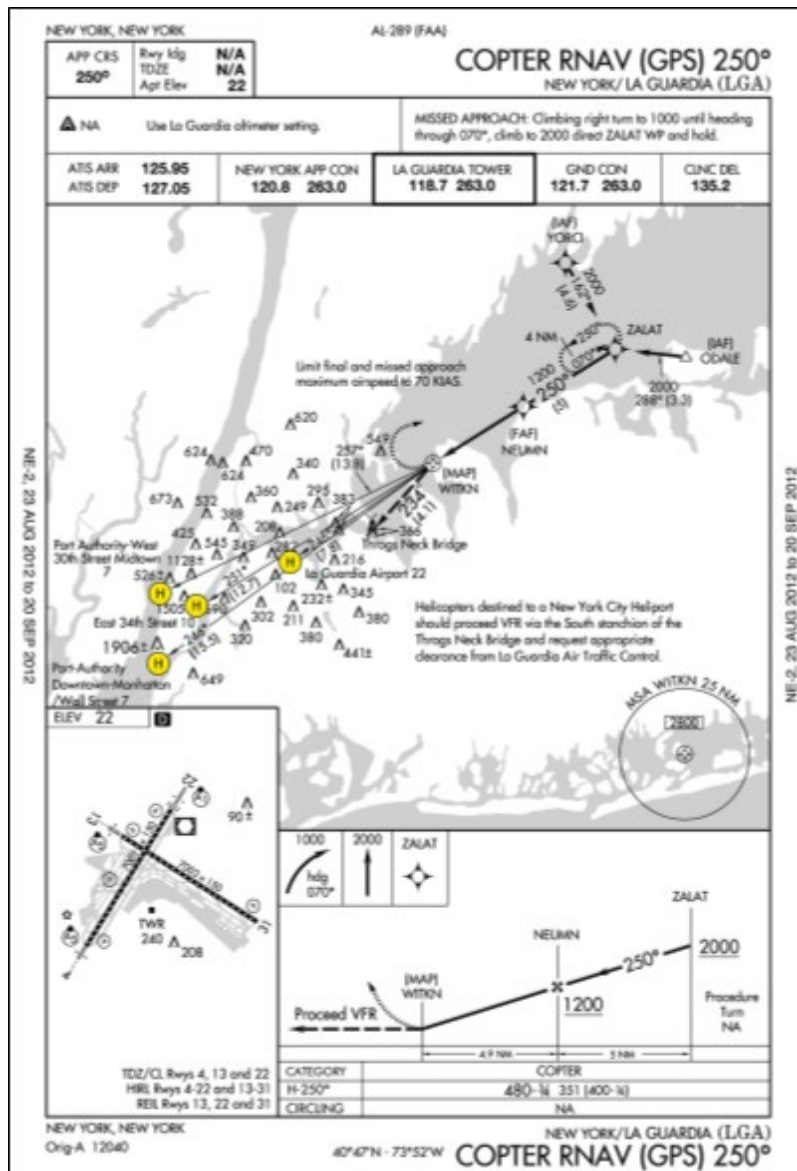
Figure 15.33. PinS Approach to Multiple Heliports.
