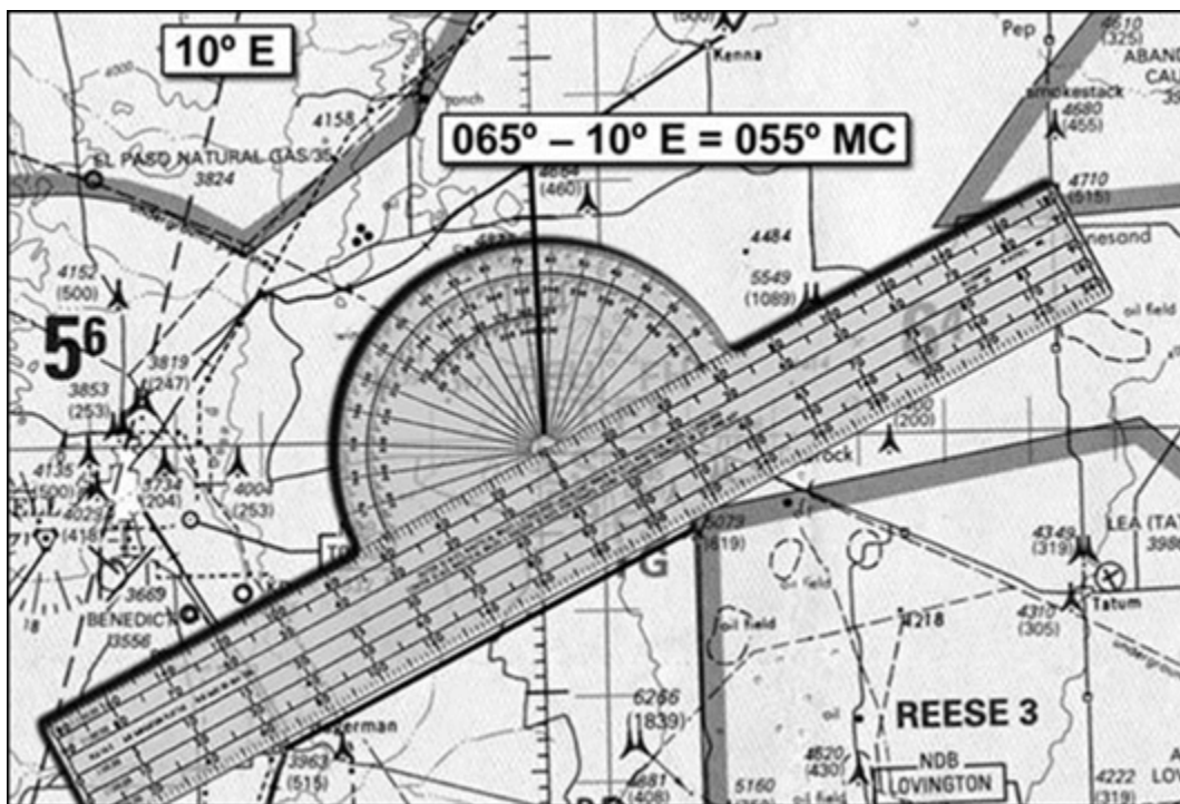
Figure 12.1. Applying Magnetic Variation.
