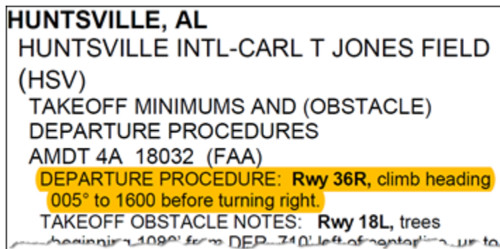
Figure 5.4. Diverse Departure Not Authorized (Runway 36R).
