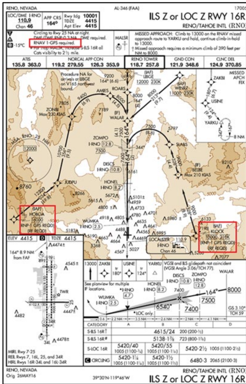
Figure 15.7. PBN Transitions to Conventional Final Approach.
