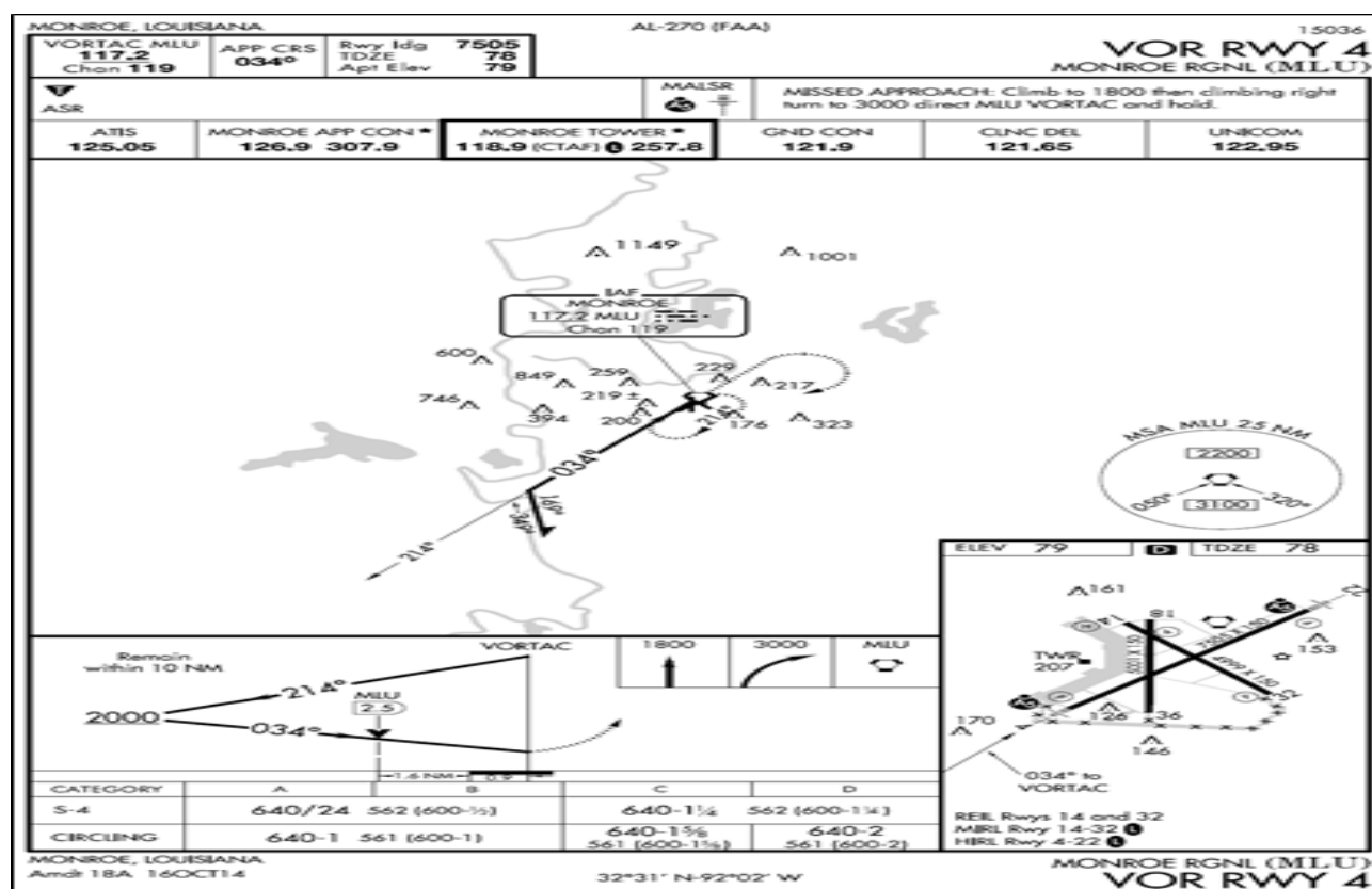
Figure 15.19. Procedure Turn with No FAF Depicted.
