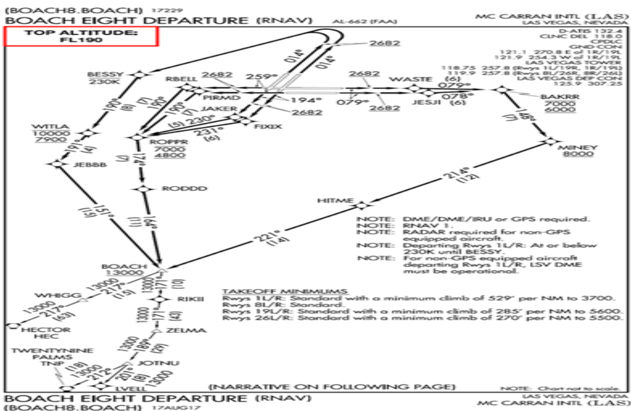
Figure 5.19. Civil SID with Top Altitude.
