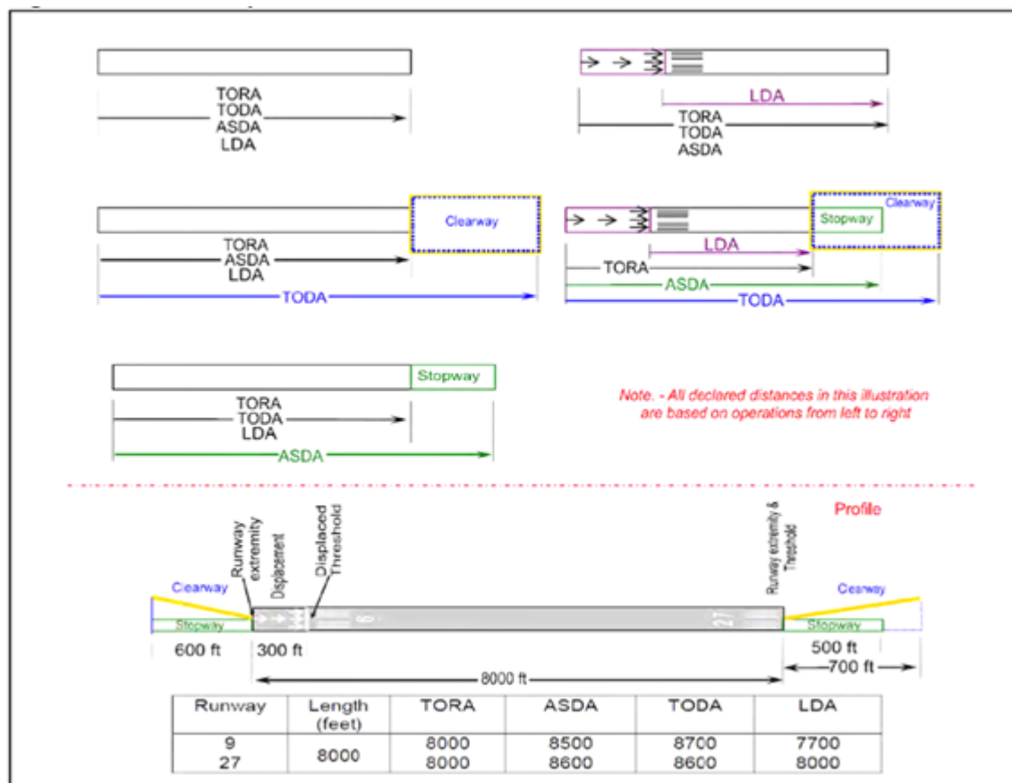
Figure 4.6. -(NAS Only) Declared Distances.
