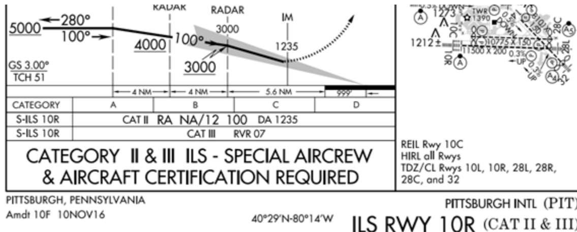
Figure 17.2. CAT II ILS Approach.
