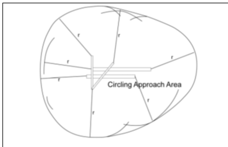
Figure 18.1. Circling Approach Area.
