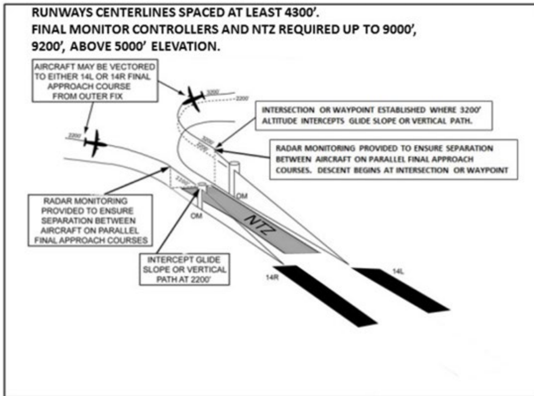
Figure 15.37. Simultaneous (Parallel) Independent Approaches.
