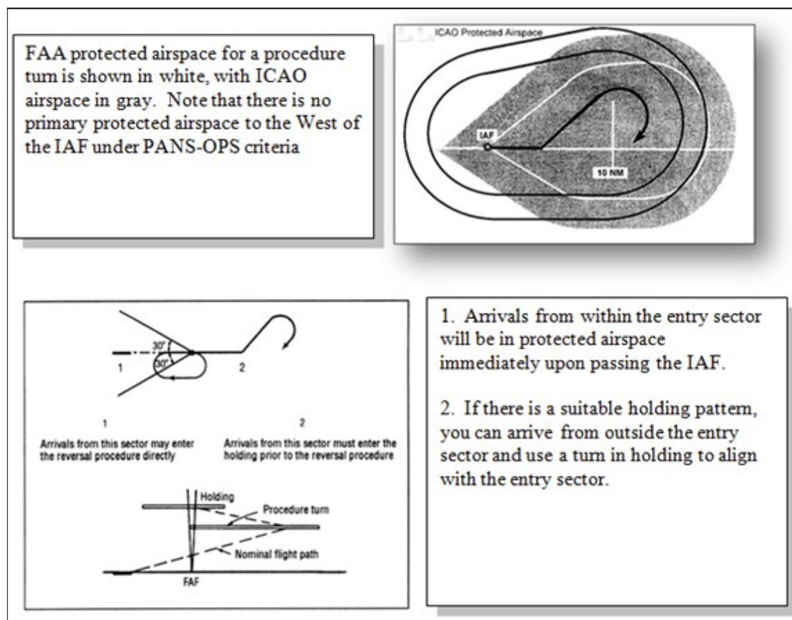
Figure 15.16. ICAO PANS-OPS versus U S TERPS Protected Airspace.
