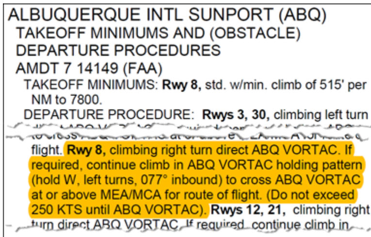
Figure 5.23. Albuquerque ODP (Runway 8).
