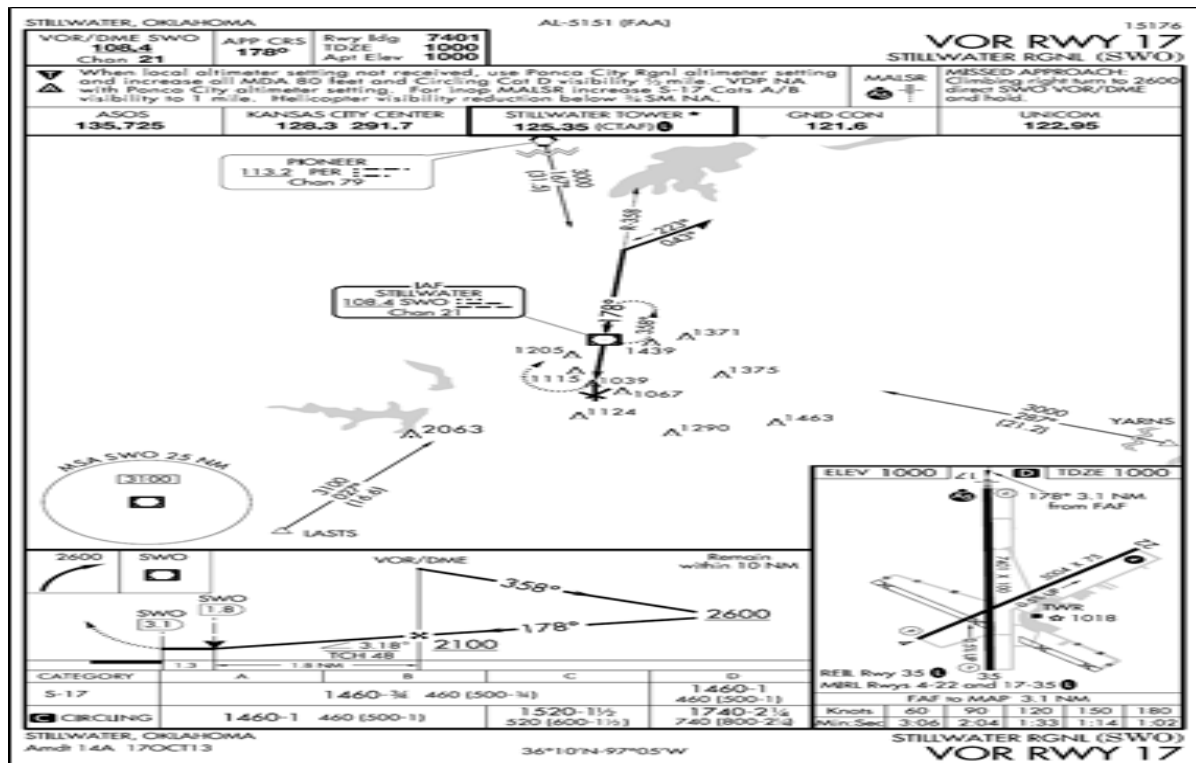
Figure 15.11. Instrument Procedure without a Charted IF.
