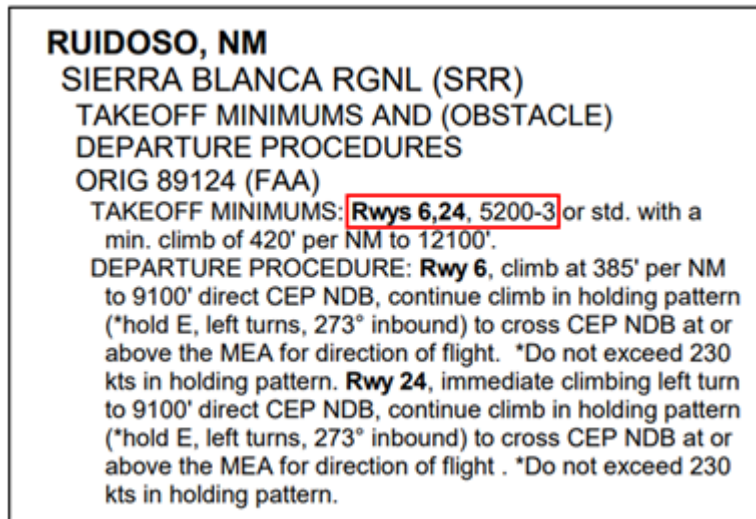
Figure 5.8. IFR Takeoff Minimums – Non –standard.
