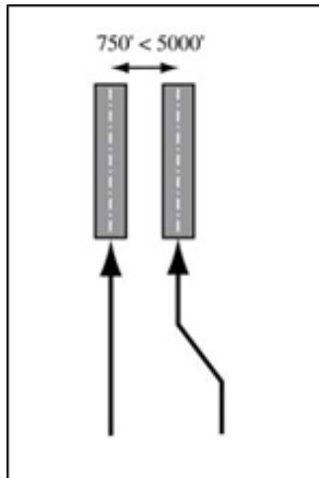
Figure 17.10. RNP Parallel Approach Runway Transition Operations.
