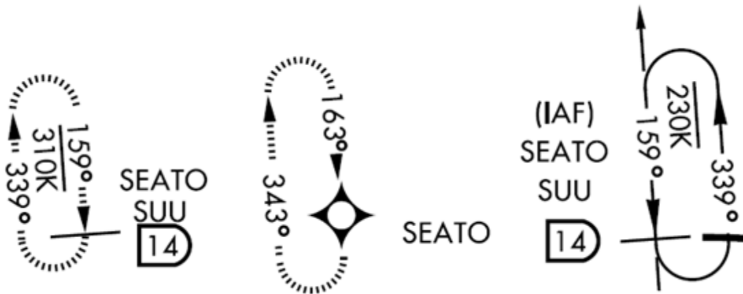
Figure 13.2. Multiple Holding Patterns at Same Fix.
