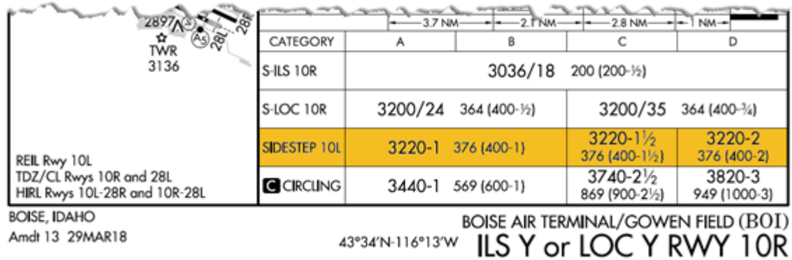
Figure 18.5. Published Side-Step Minimums.
