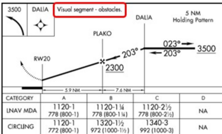
Figure 16.2. Visual Segment – Obstacles.
