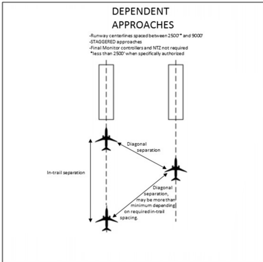
Figure 15.36. Simultaneous Dependent Approaches.
