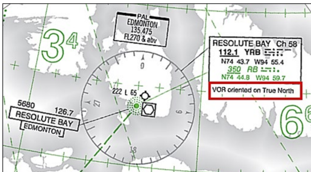
Figure 20.2. Enroute Charts for Navigation at Higher Latitudes.
