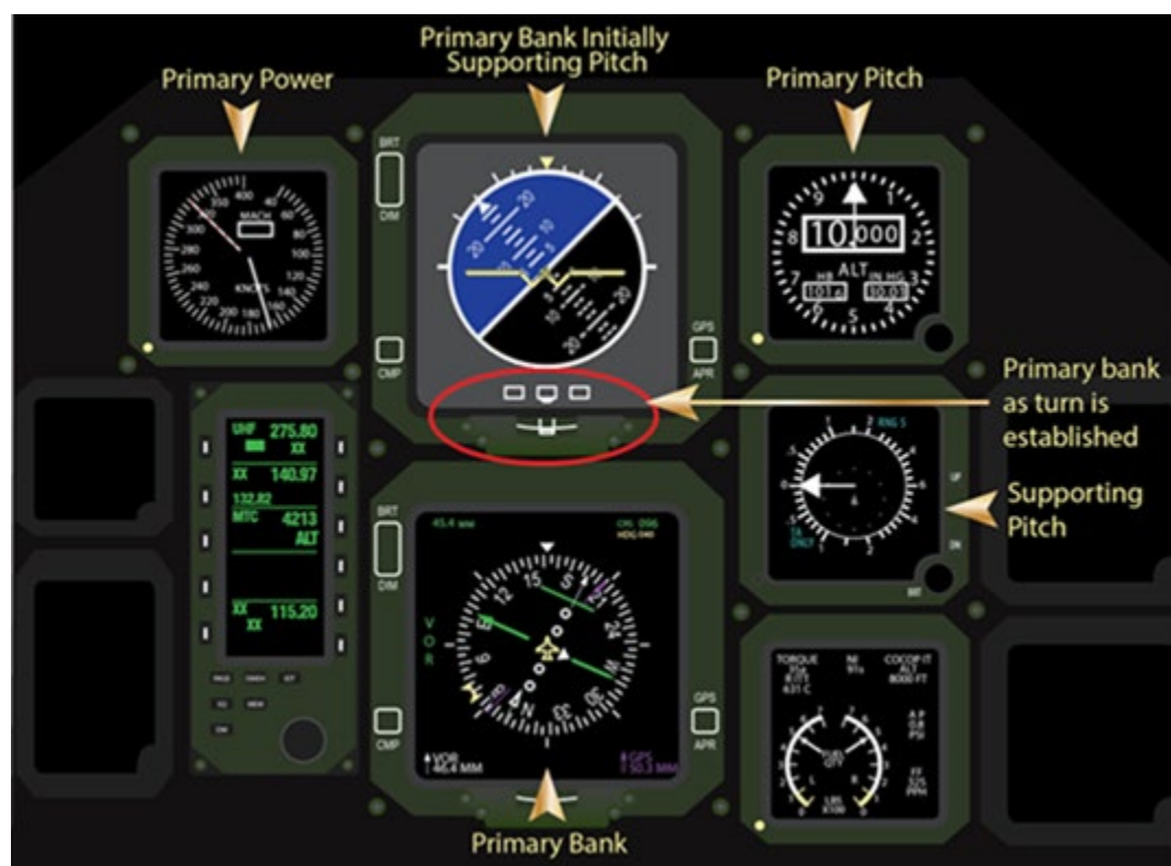
Figure A5.4. Level Turns.
