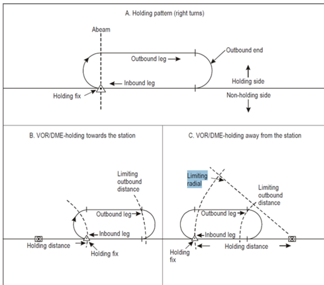
Figure 13.5. ICAO Limiting Radial.
