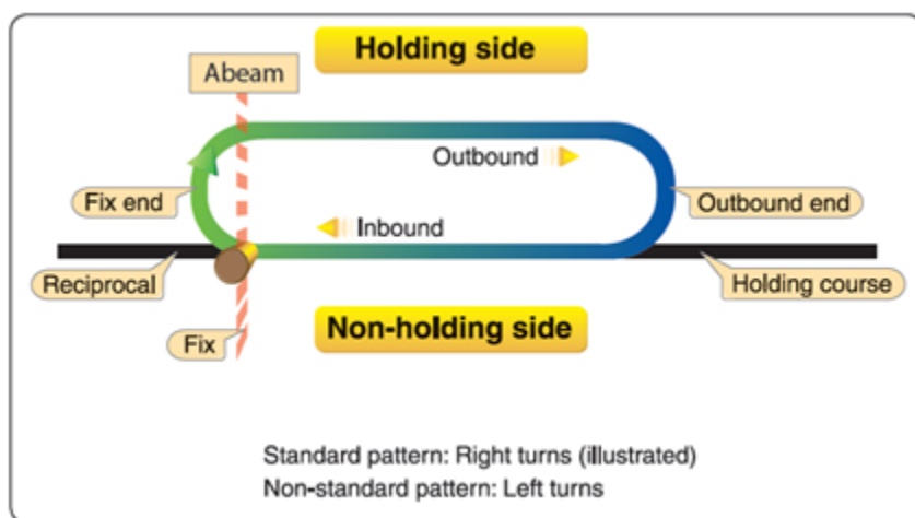
Figure 13.1. Standard Holding Pattern.
