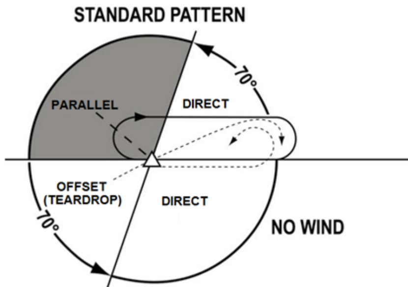
Figure 13.3. Holding Entry Sectors.
