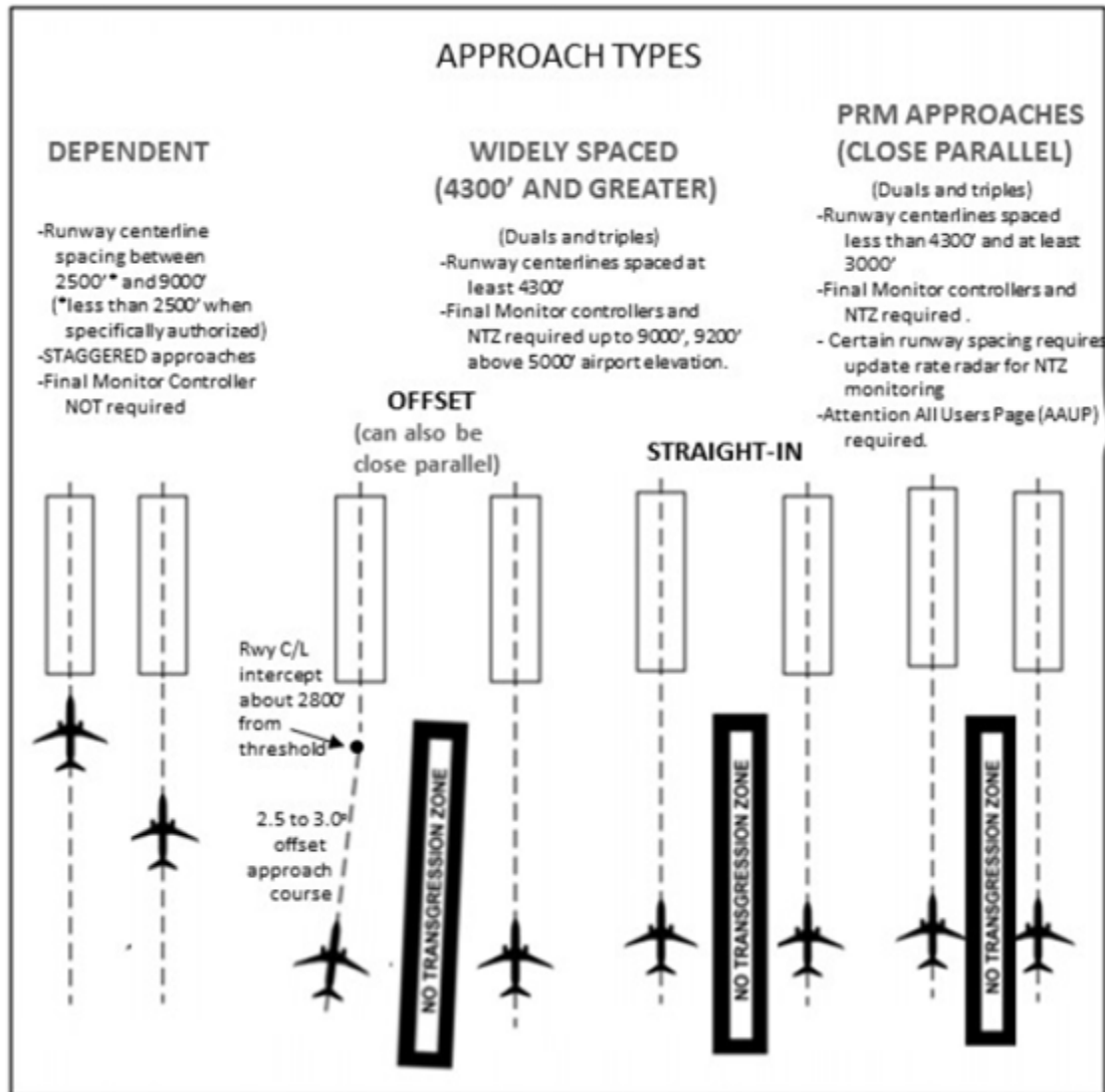
Figure 15.35. Simultaneous Approaches to Parallel Runways.
