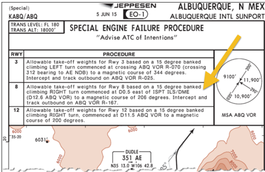
Figure 5.24. Albuquerque SDP (Runway 8).
