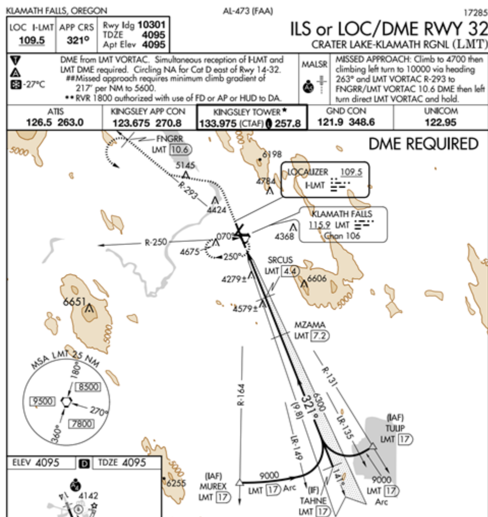
Figure 15.18. Procedure Turn Not Authorized.
