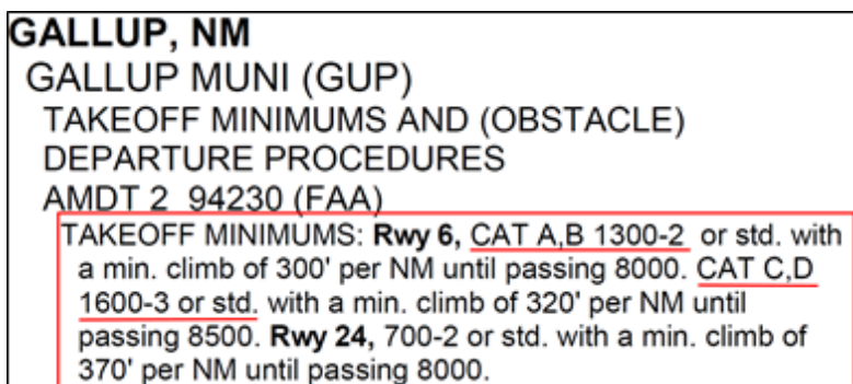
Figure 5.10. IFR Takeoff Minimums – Specific Aircraft Category.
