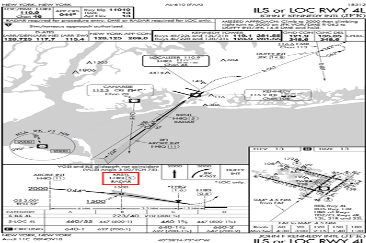
Figure 15.6. Radar Fix on Non-radar Approach.
