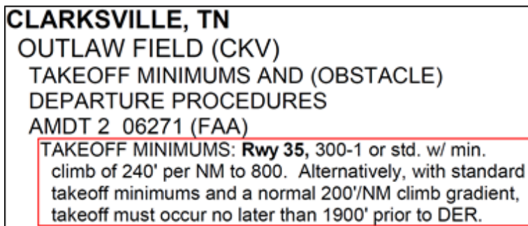
Figure 5.9. IFR Takeoff Minimums – “Or Standard”.
