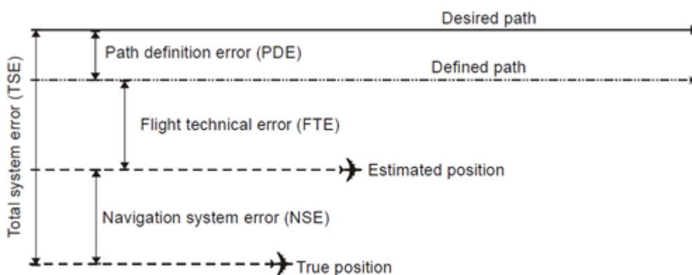
Figure 6.3. Lateral Navigation Errors.
