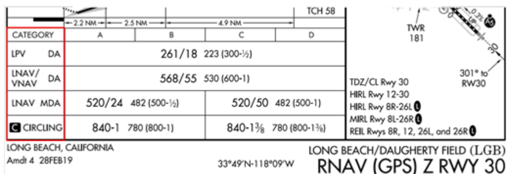
Figure 15.8. RNAV Lines of Minima.
