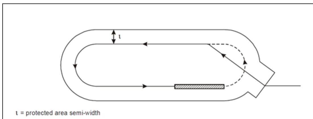
Figure 18.4. Visual Maneuver Using a Prescribed Track Protected Area.
