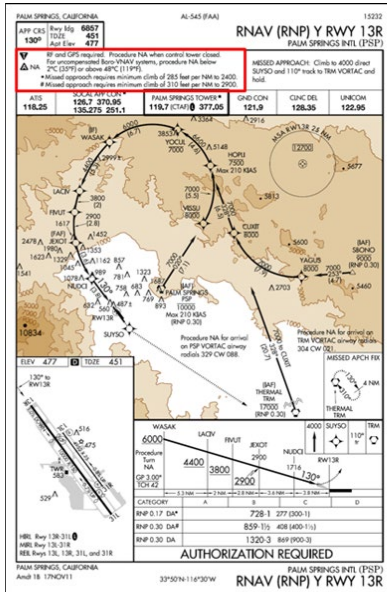
Figure 17.7. Nonstandard Missed Approach Climb Gradient.
