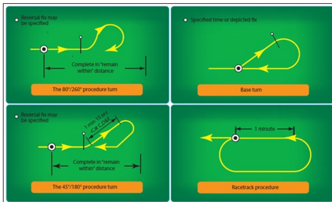
Figure 15.13. Types of Course Reversals.
