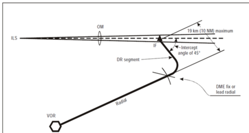
Figure 15.12. -(ICAO) Dead Reckoning Segment.
