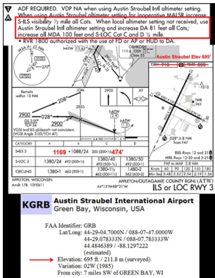
Figure 4.13. Cold Temperature Corrections – Remote Altimeter Setting.
