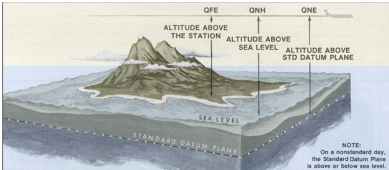
Figure 4.8. Types of Altimeter Settings.
