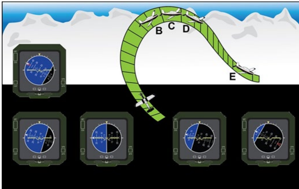
Figure A5.8. Wingover.
