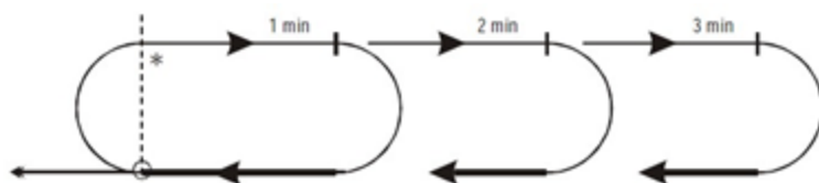
Figure 15.25. Racetrack or [NAS Only] HILPT.
