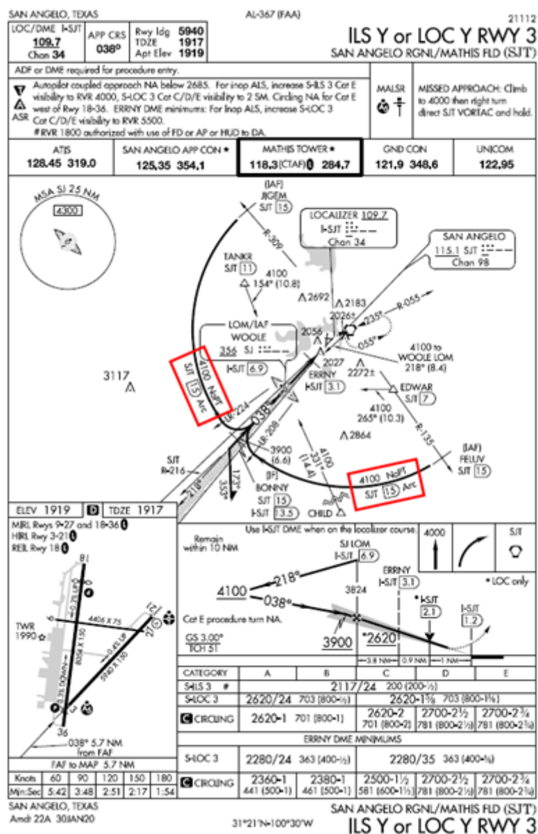
Figure 15.27. [NAS Only] NoPT Routing.
