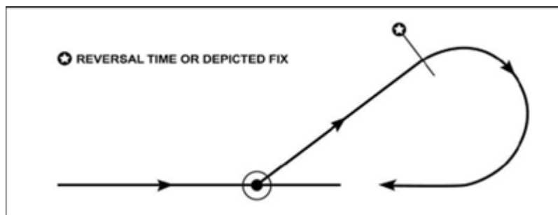
Figure 15.24. Base Turn with More Than One Track.
