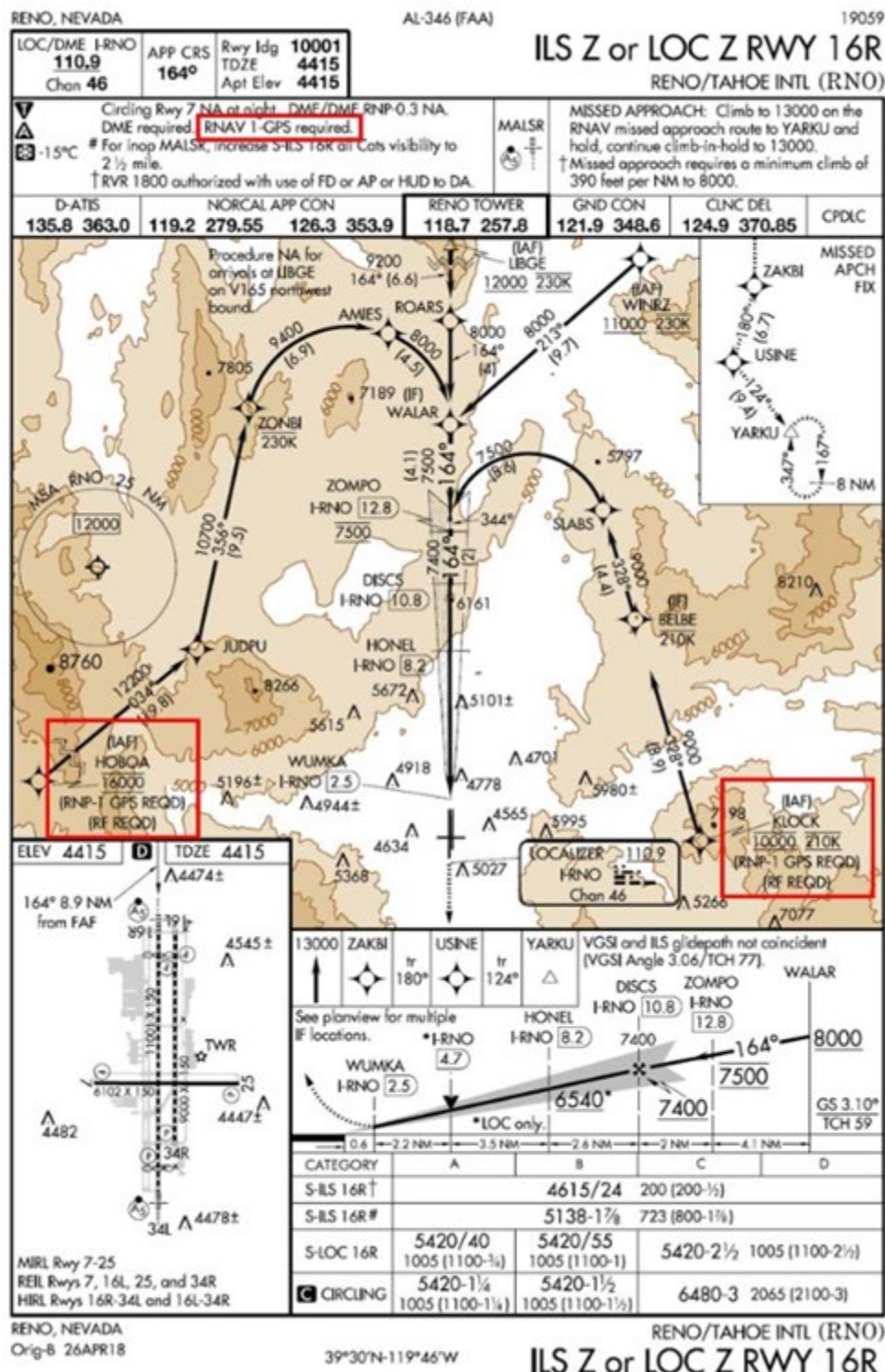
Figure 15.7. PBN Transitions to Conventional Final Approach.
