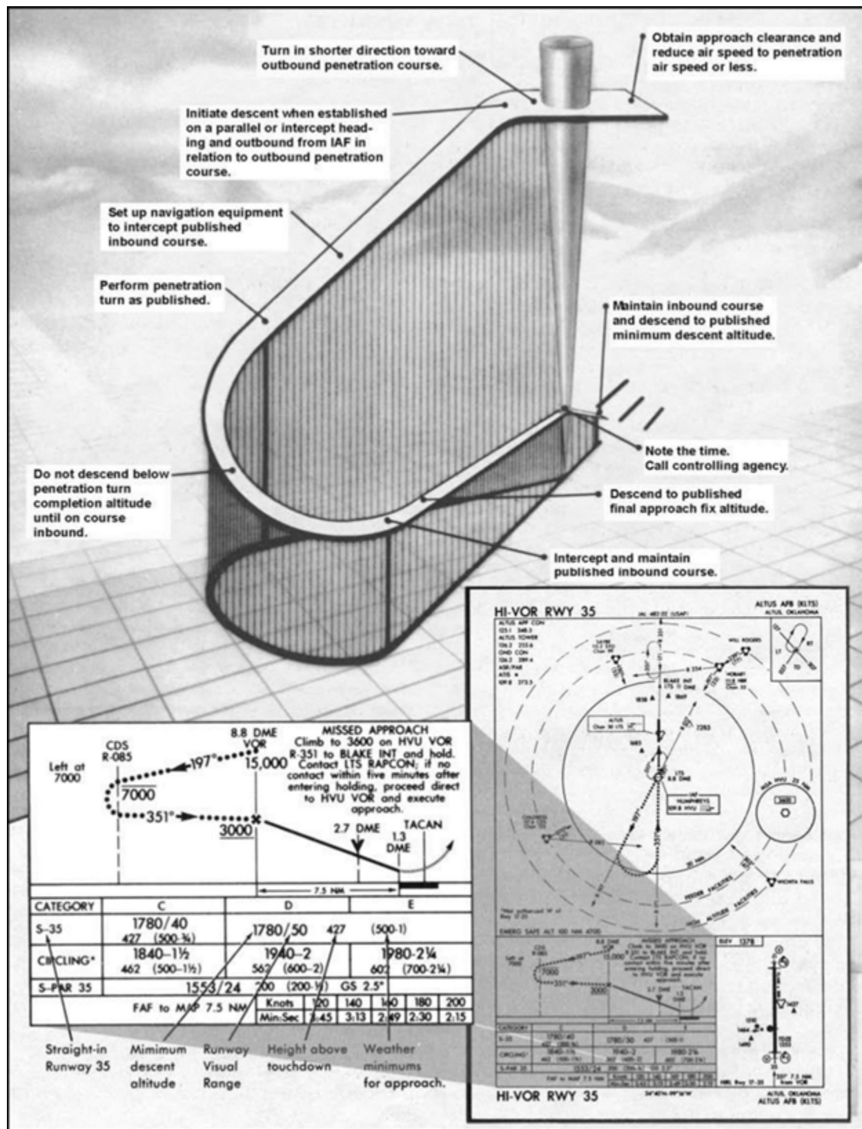
Figure 15.29. Non-DME Teardrop High Altitude Approach.
