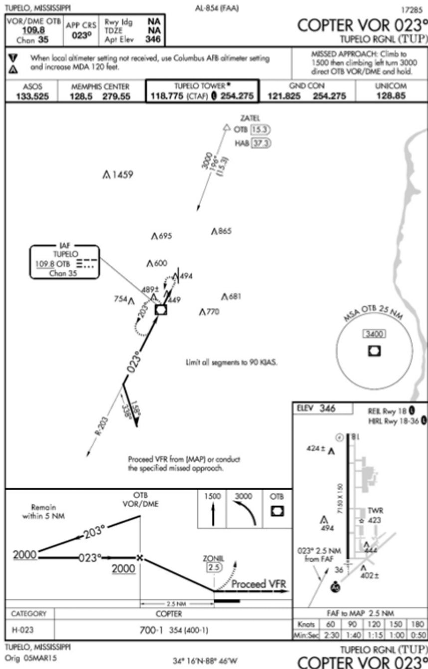
Figure 15.32. Point-in-Space (PinS) Approach.
