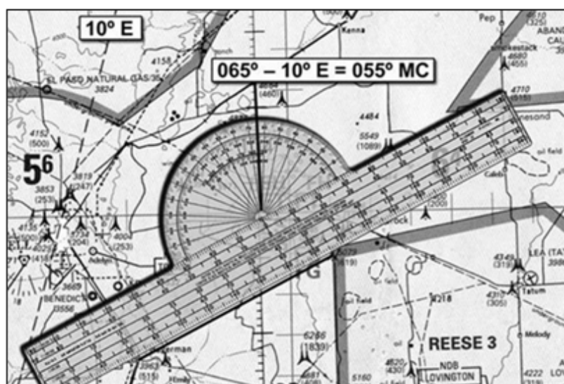
Figure 12.1. Applying Magnetic Variation.
