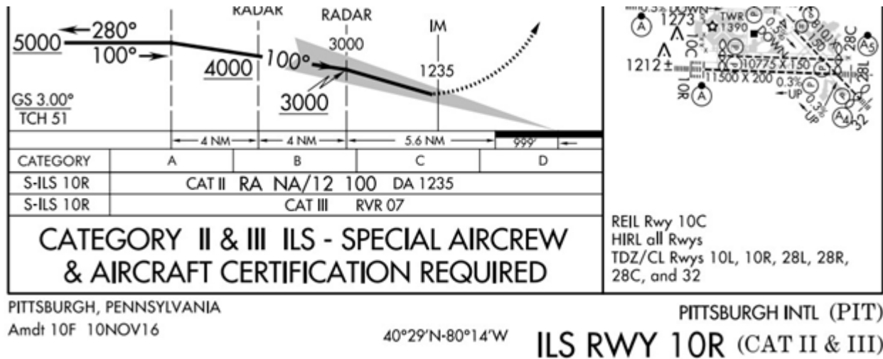
Figure 17.2. CAT II ILS Approach.
