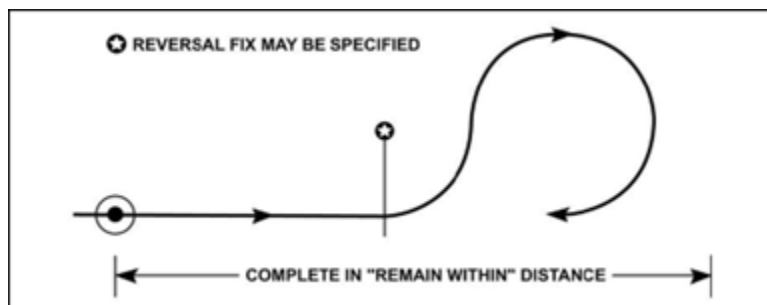
Figure 15.22. 80°/260° Procedure Turn.
