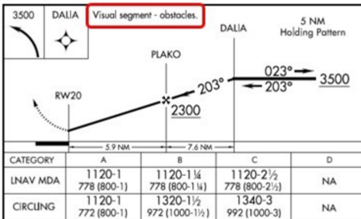
Figure 16.2. Visual Segment – Obstacles.
