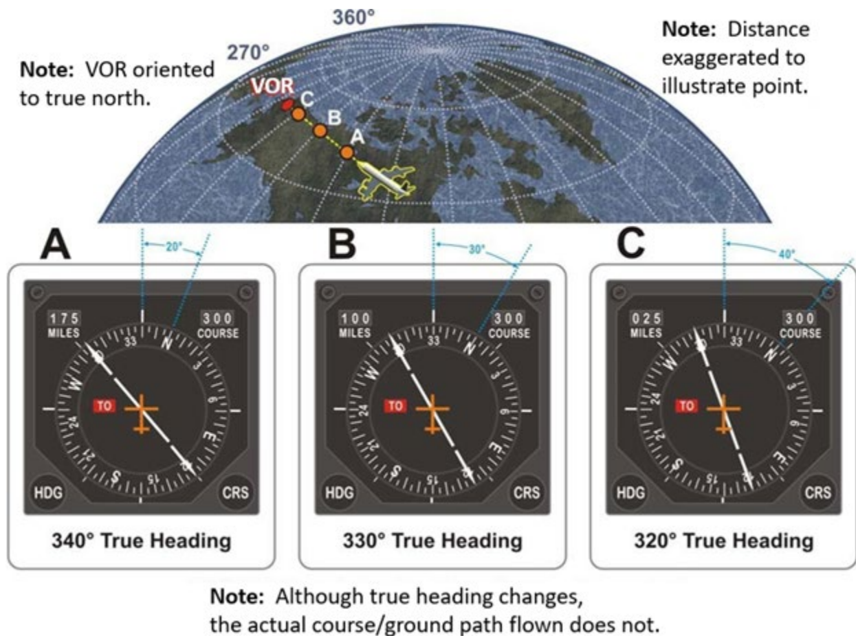
Figure 20.1. Heading Indications While Crossing Meridians.
