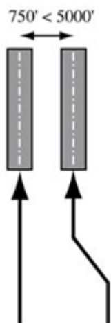
Figure 17.10. RNP Parallel Approach Runway Transition Operations.
