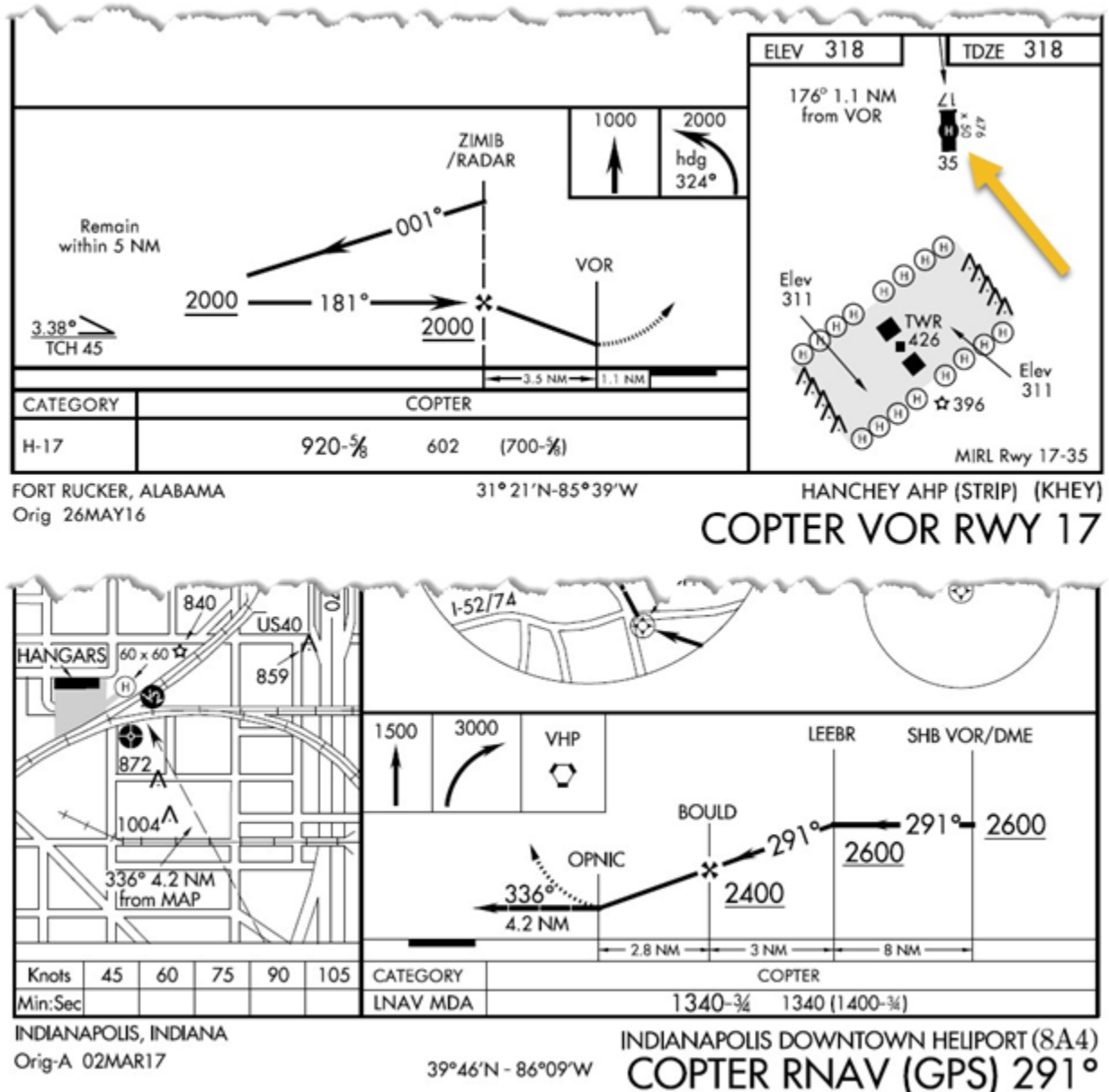
Figure 15.30. Helicopter-Only Approach.
