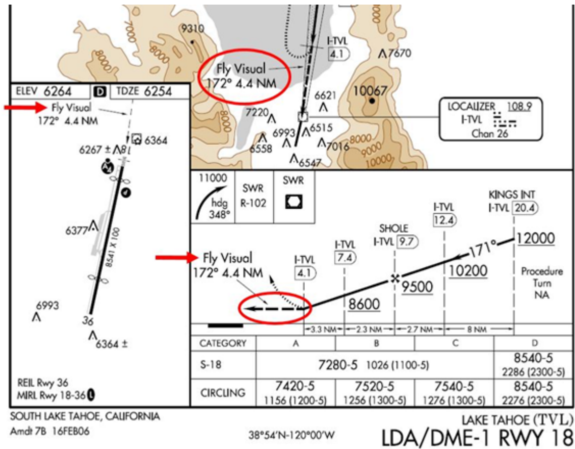
Figure 16.10. Visual Segment.
