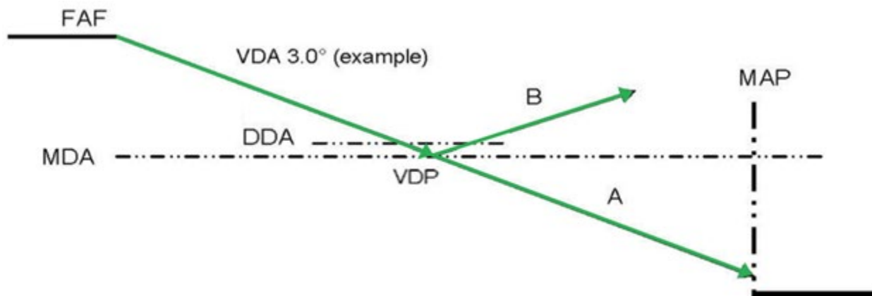
Figure 16.5. CDFA.
