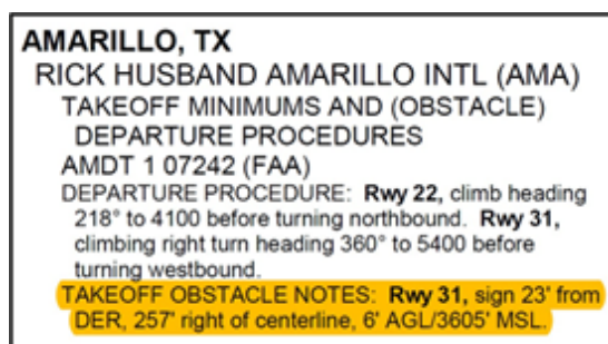
Figure 5.2. Low Close-in Obstacles.
