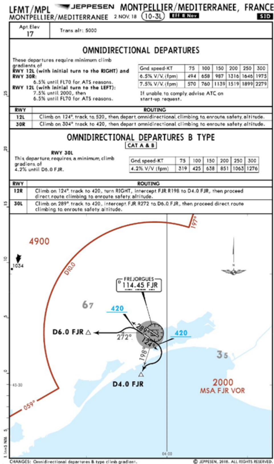
Figure 5.6. Omnidirectional Departure.
