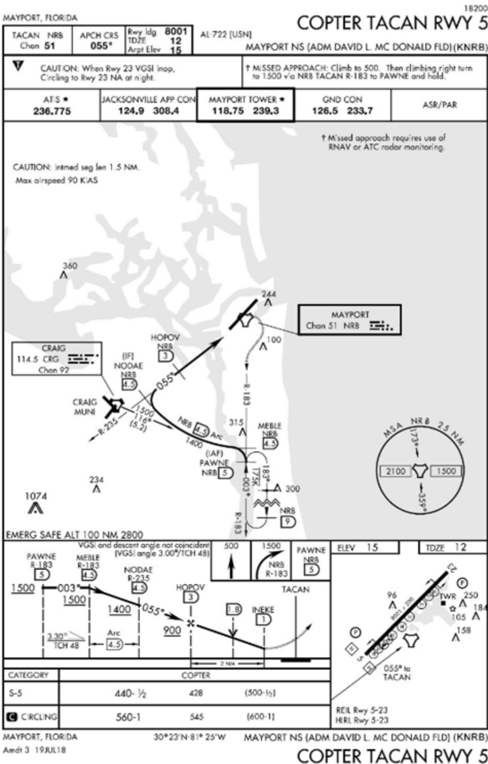
Figure 15.31. Short Final Approach.
