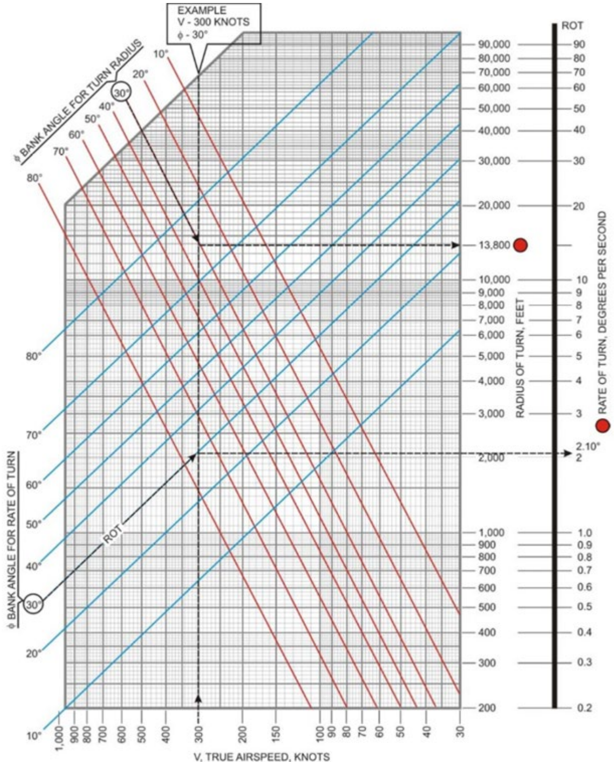
Figure A3.1. General Turning Performance (Constant Altitude, Steady Turn).
