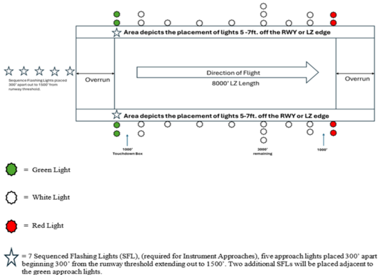
Figure 4.4. (PACAF) AMP-1F, Night.
