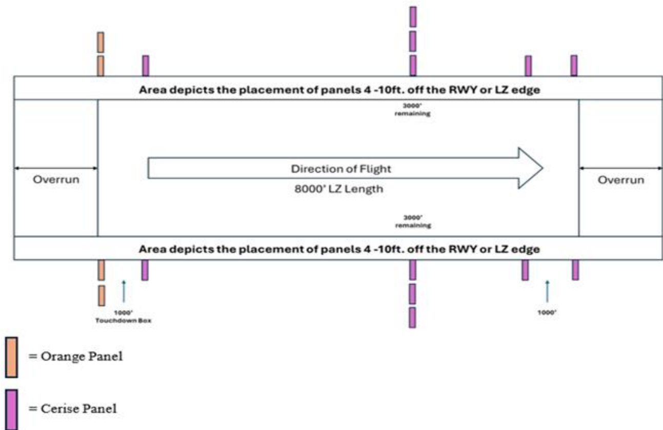
Figure 4.5. (PACAF) AMP-2 Day.
