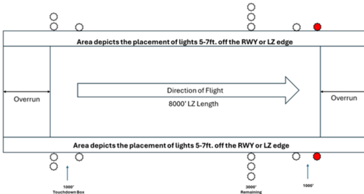
Figure 4.6. (PACAF) AMP-2 Night.
