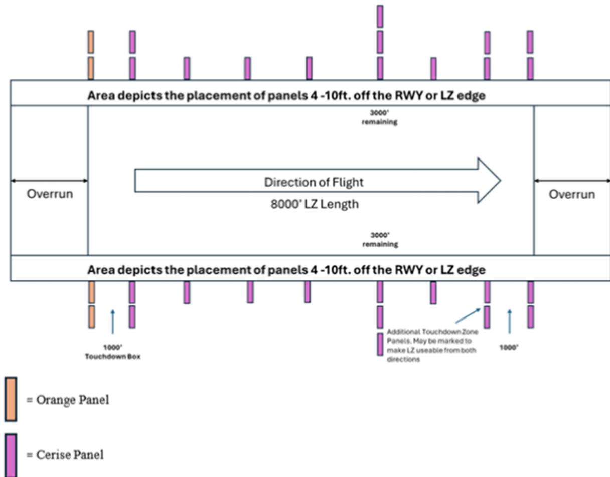
Figure 4.3. (PACAF) AMP-1F, Day.
