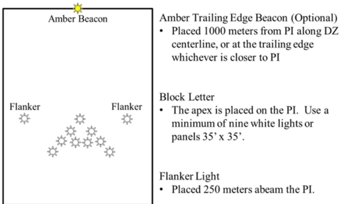
Figure 3.3. Standard DZ Markings.
