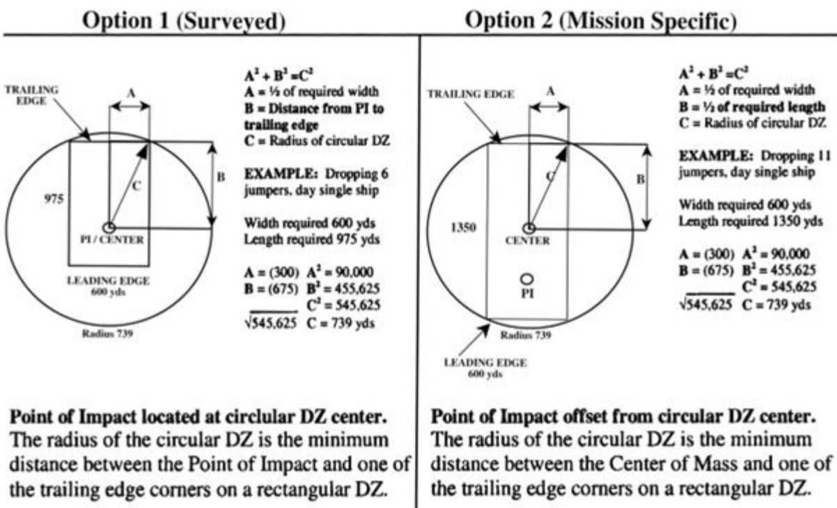
Figure 3.1. Circular DZ Computation.
