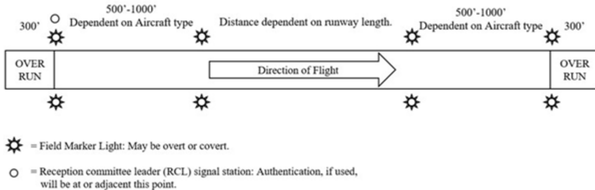
Figure 4.6. (PACAF) AMP-2 Night.
